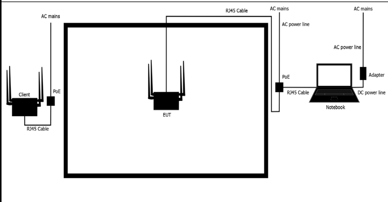
Test Setup Diagram - Radiated Test (mode 8)
