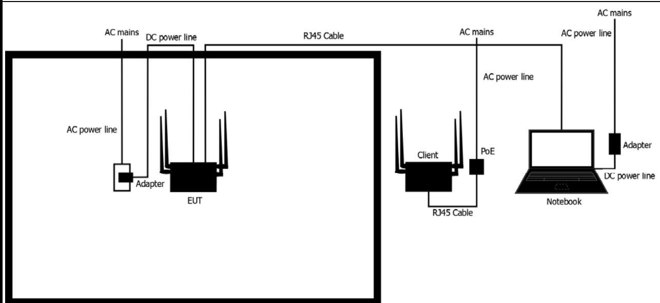
Test Setup Diagram - Radiated Test (mode 7)
