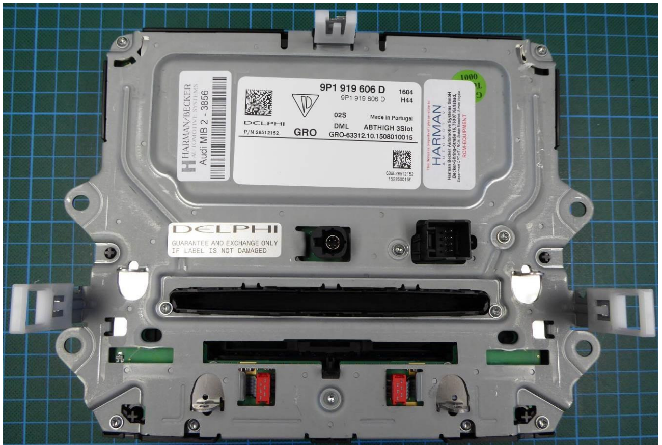
160090_07. jpg: EUT – Front panel back view
