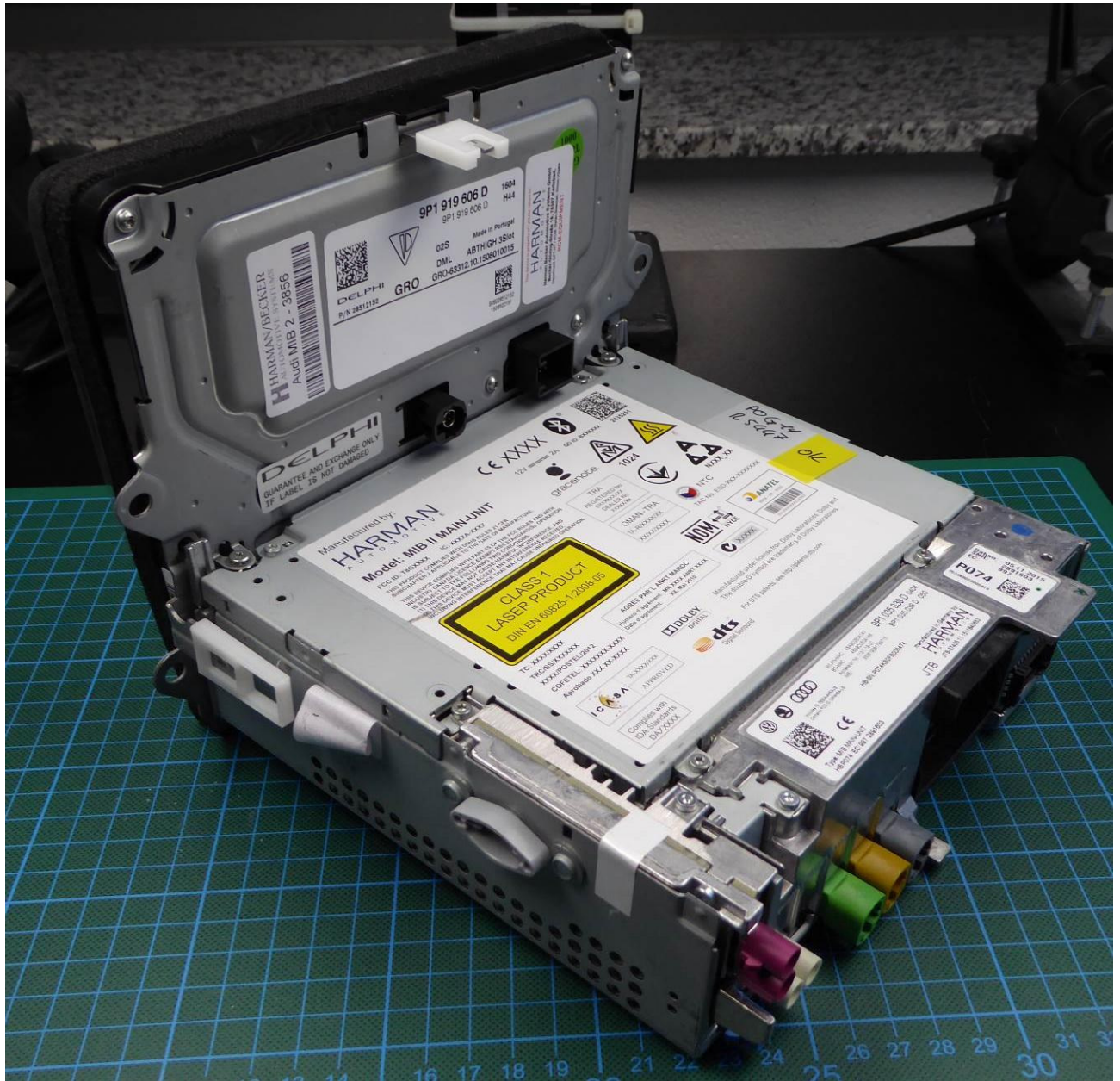
160090_05. jpg: EUT – 3D back view 2
