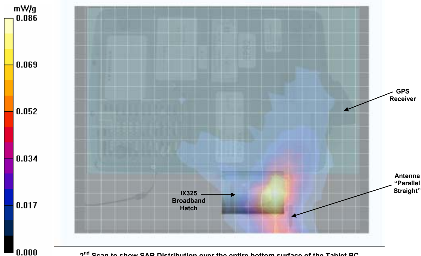
2 nd Scan to show SAR Distribution over the entire bottom surface of the Tablet PC
