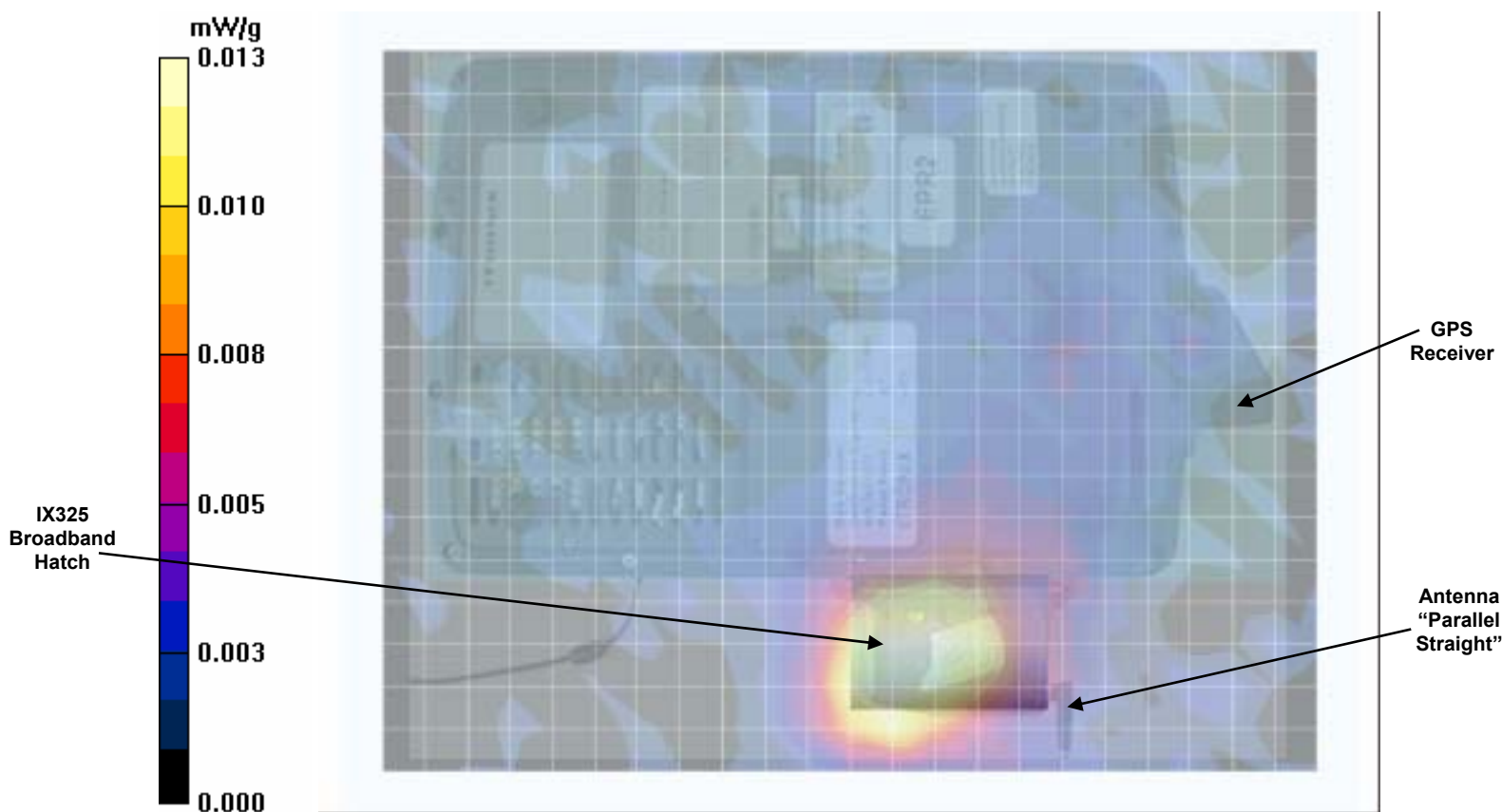
2 nd Scan to show SAR Distribution over the entire bottom surface of the Tablet PC
