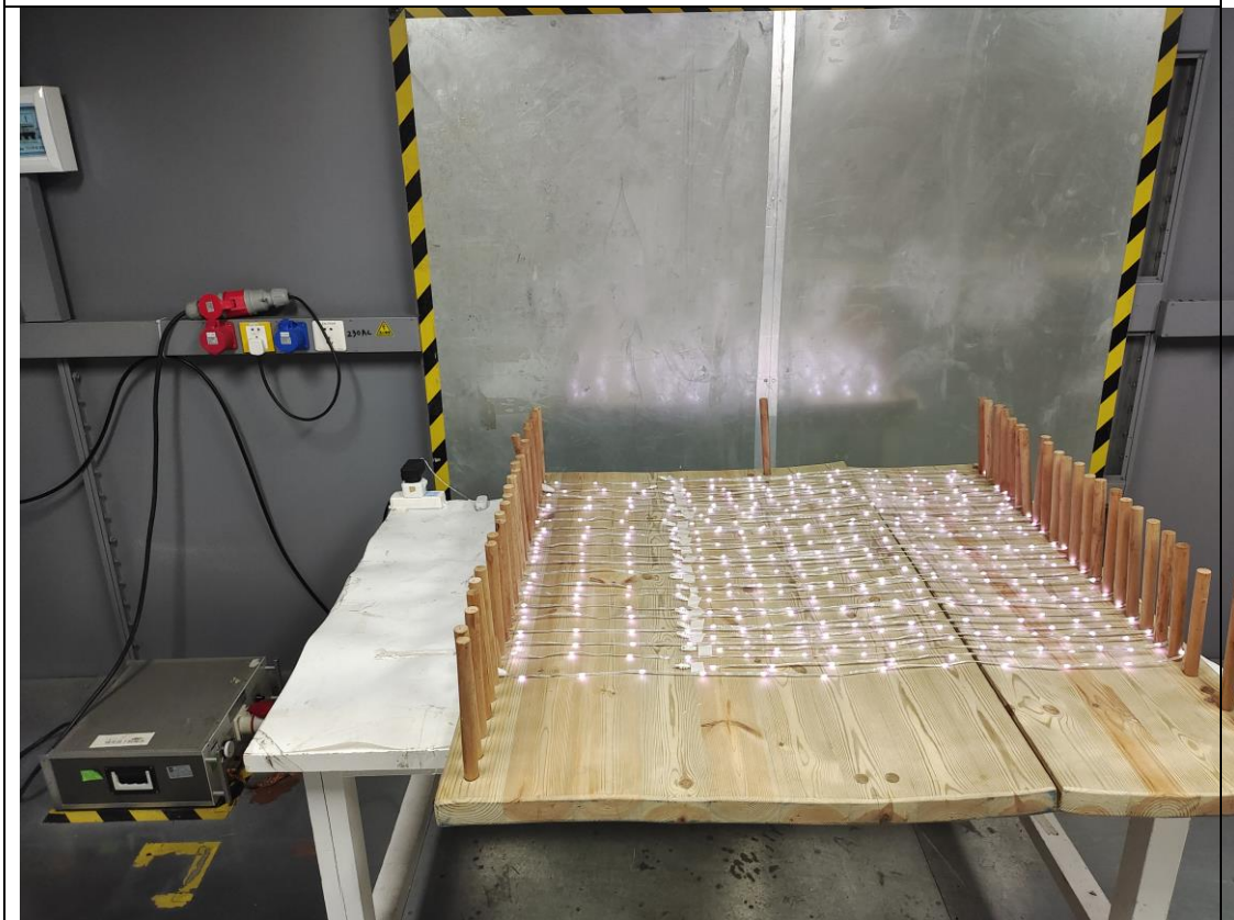
Conducted emission
