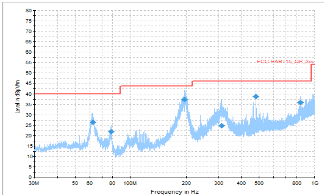
Figure A.1.53. Radiated Emission (Data Transfer: TF Card TO PC, 30MHz to 1GHz) Final_Results
