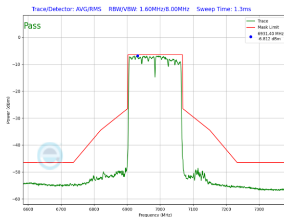
Plot 7-896. LPI In-Band Emission Plot SDM Antenna WF7a (160MHz 802.11ax RU996x2 (UNII Band 8) – Ch. 207)
