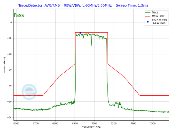
Plot 7-895. LPI In-Band Emission Plot SDM Antenna WF8 (160MHz 802.11ax RU996x2 (UNII Band 8) – Ch. 207)
