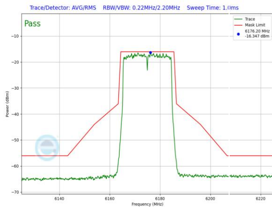
Plot 7-776. LPI In-Band Emission Plot SDM Antenna WF8 (20MHz 802.11ax RU242 (UNII Band 5) – Ch. 45)
