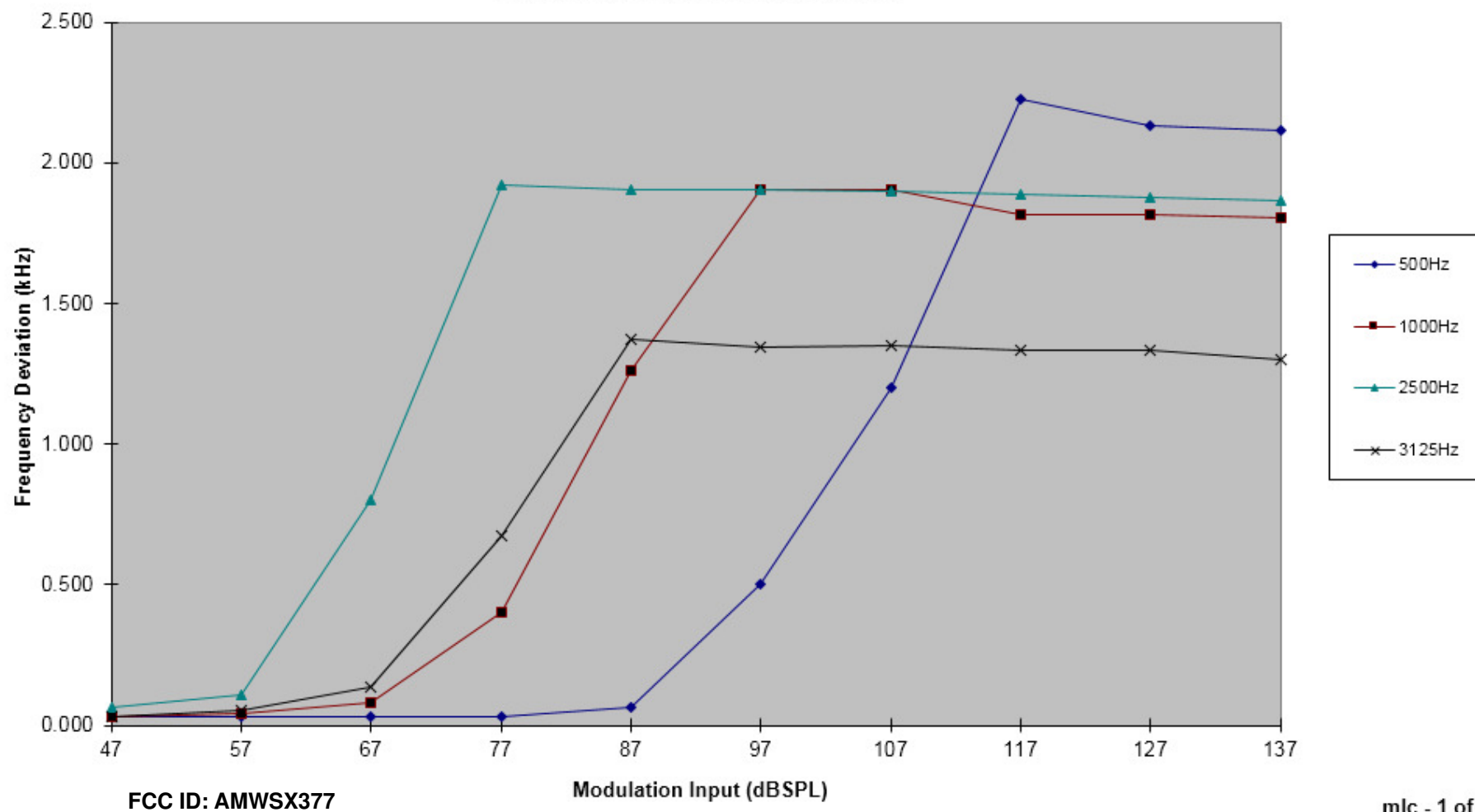
INTERTEK TESTING SERVICES Modulation Limiting Characteristic
