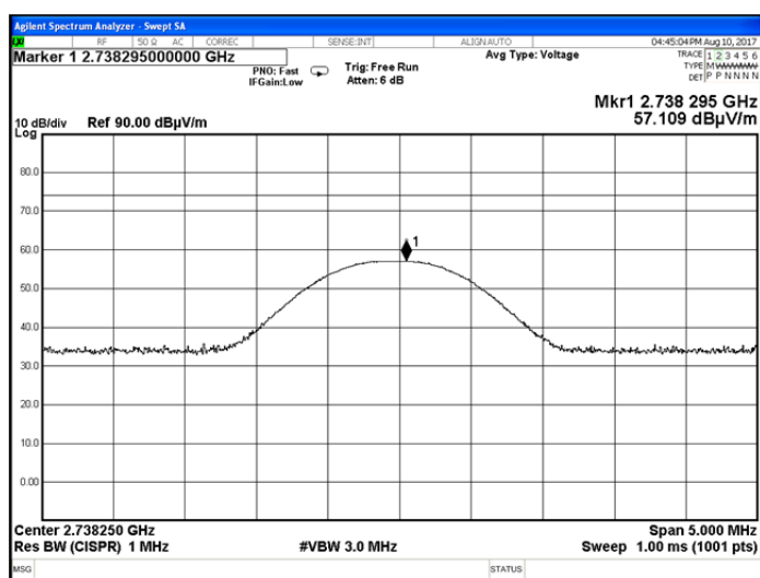
Plot 7.6.22 Radiated emission measurements at the third harmonic of low carrier frequency
