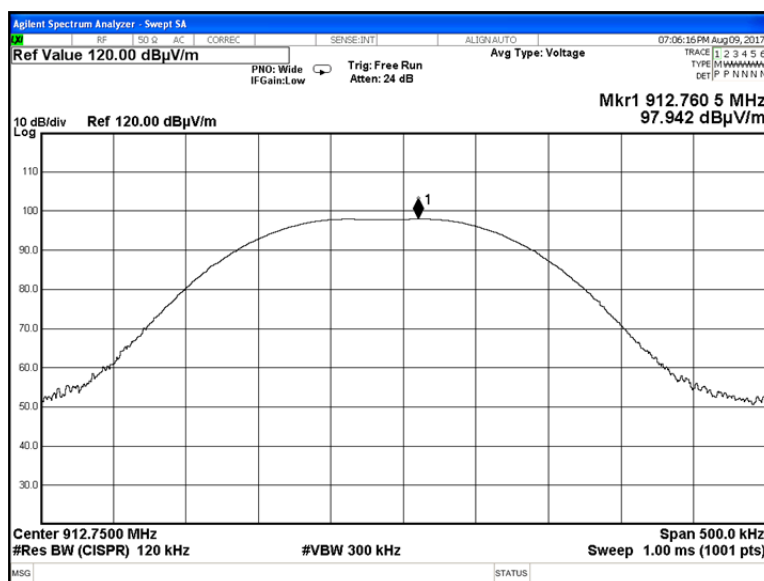
Plot 7.5.4 Field strength of carrier at low frequency and Unom
