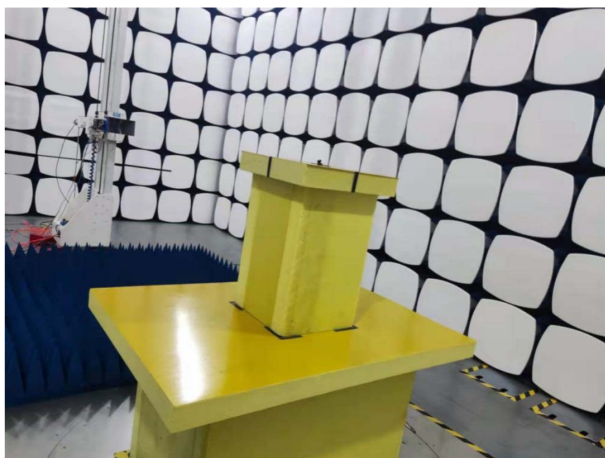
Above 1GHz(BT)
