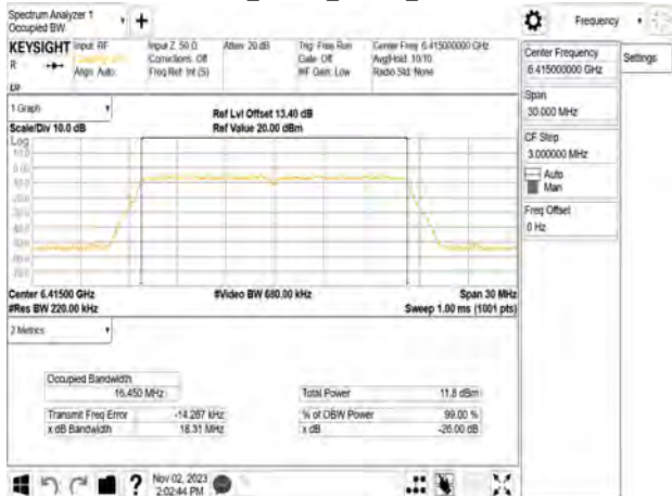
802.11a_20MHz_Chain0_6415MHz
