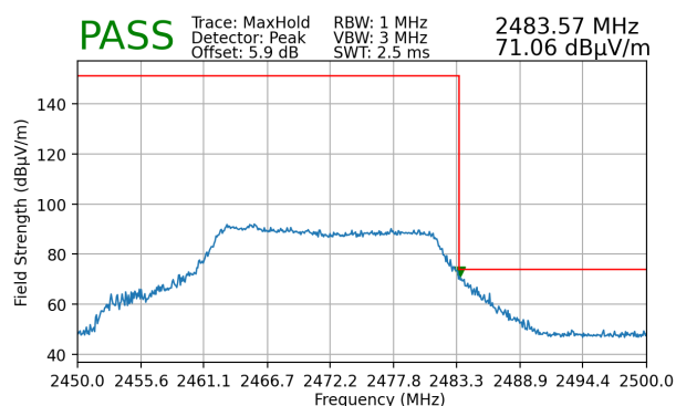
Plot 7-113. Radiated Restricted Upper Band Edge Measurement (Peak)
