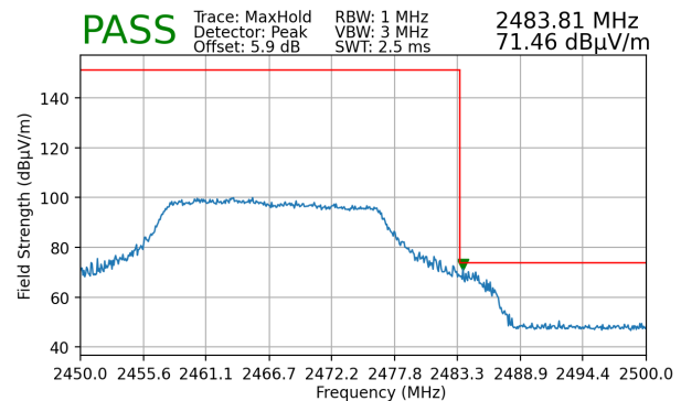
Plot 7-111. Radiated Restricted Upper Band Edge Measurement (Peak)
