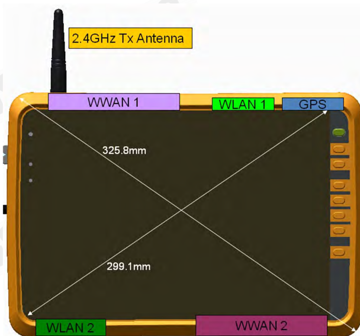
Front view of the tablet with transceiver attached
