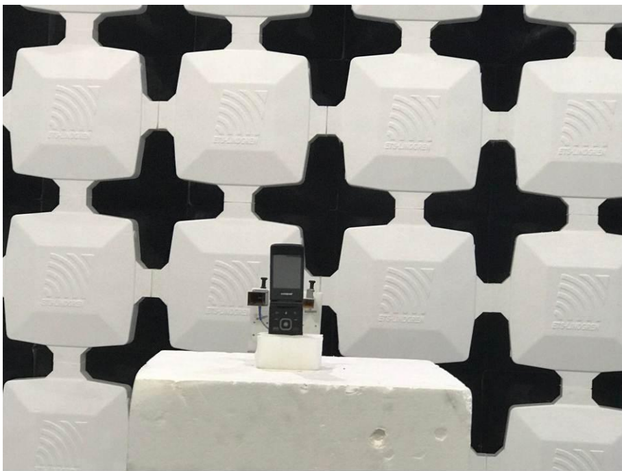
10. Radiated Emissions (Part 22/24) (Above 18GHz)
