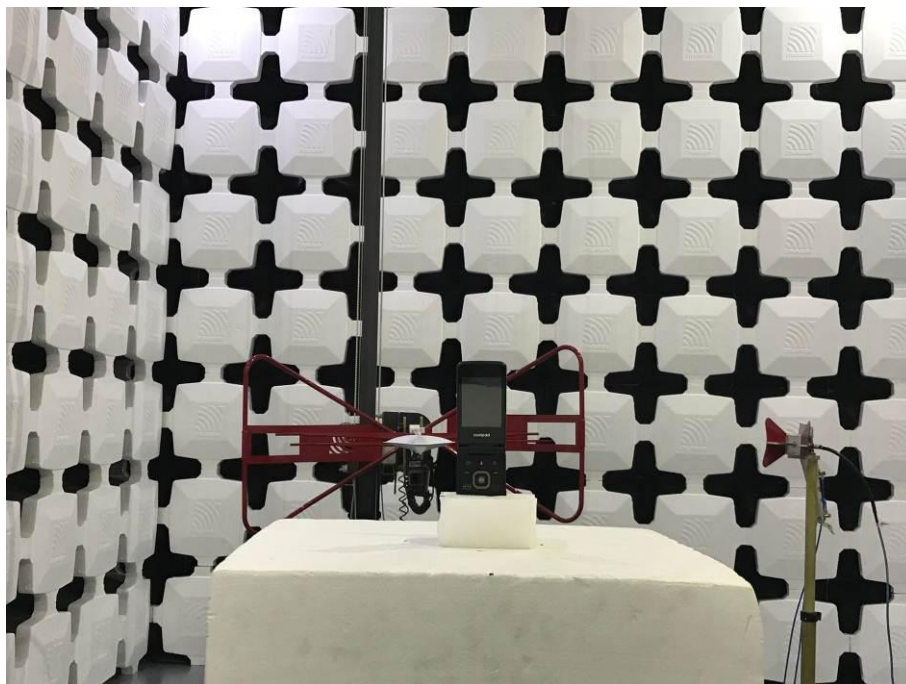
6. Radiated Emissions (Part 15C&15E 30M-18GHz)
