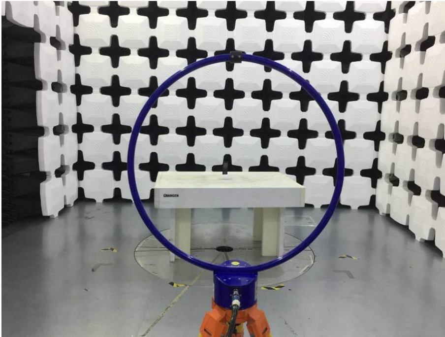
5. Radiated Emissions (Part 15C&15E 9kHz-30MHz)
