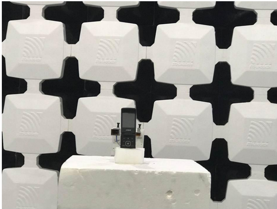
7. Radiated Emissions (Part 15C&15E) (18GHz-40GHz)
