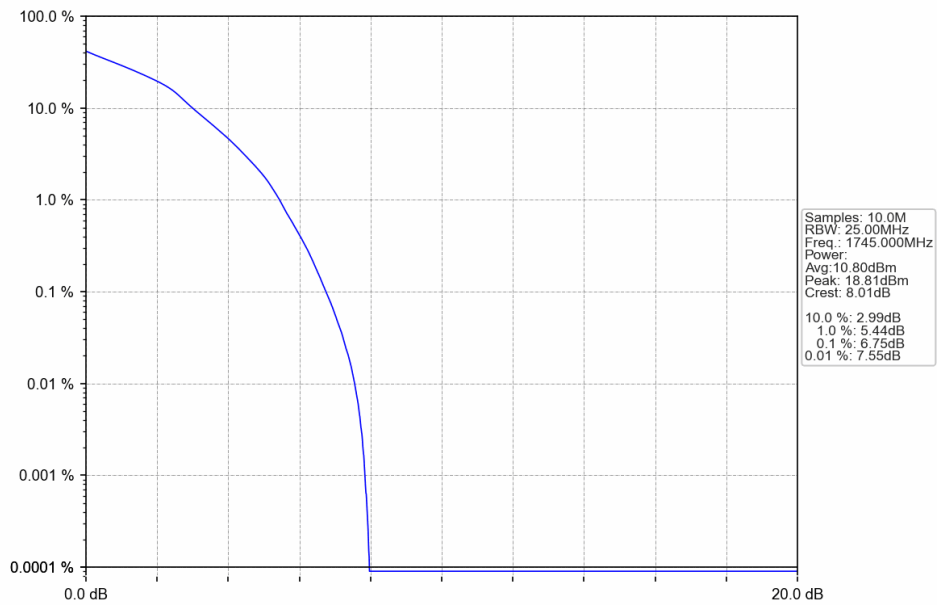
Band4_20MHz_16QAM_HCH_1745MHz_RB_27_73_NTNV
