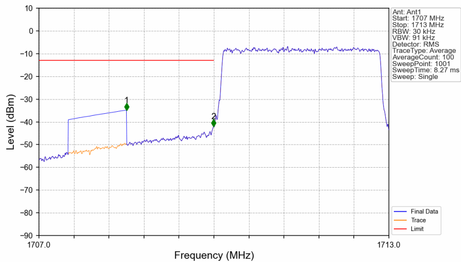
Band4_3MHz_16QAM_LCH_1711.5MHz_RB_15_0_NTNV
