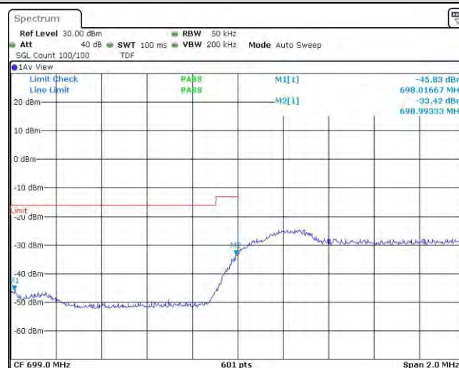
Band12-3MHz-16QAM-23025-15RB#0
