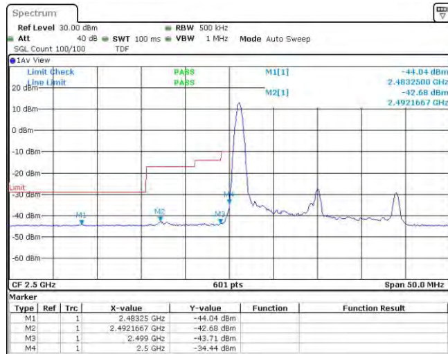
Band7-20MHz-16QAM-20850-1RB#99
