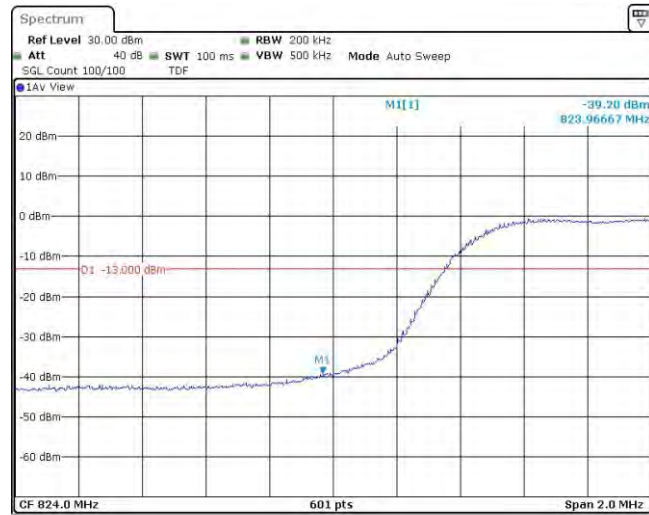
Band5-10MHz-QPSK-20450-1RB#49
