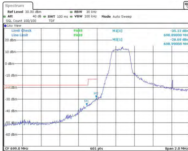
Band12-1.4MHz-16QAM-23017-1RB#5
