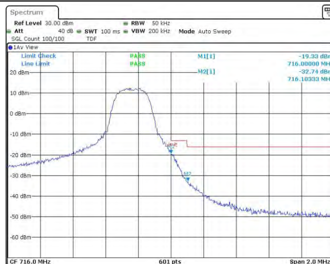
Band12-3MHz-16QAM-23165-15RB#0
