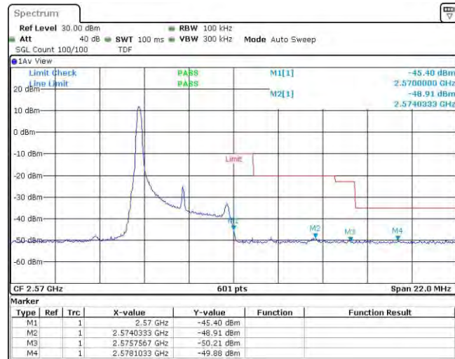
Band7-5MHz-16QAM-21425-1RB#24
