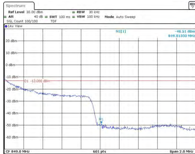
Band5-1.4MHz-16QAM-20643-1RB#5
