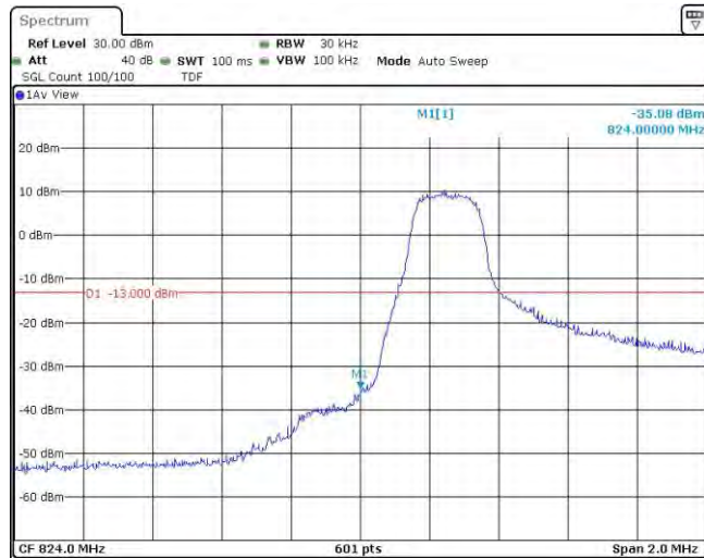
Band5-1.4MHz-QPSK-20407-1RB#5
