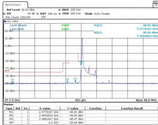
Band7-5MHz-QPSK-20775-1RB#24
