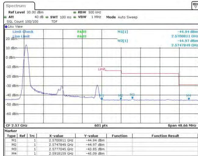
Band7-20MHz-16QAM-21350-1RB#99
