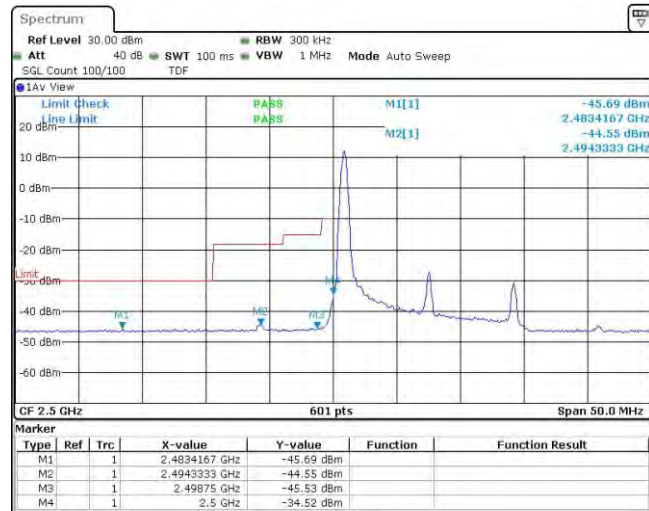
Band7-15MHz-QPSK-20825-1RB#74
