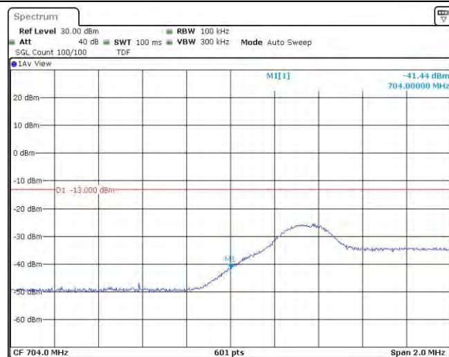
Band17-5MHz-QPSK-23755-25RB#0
