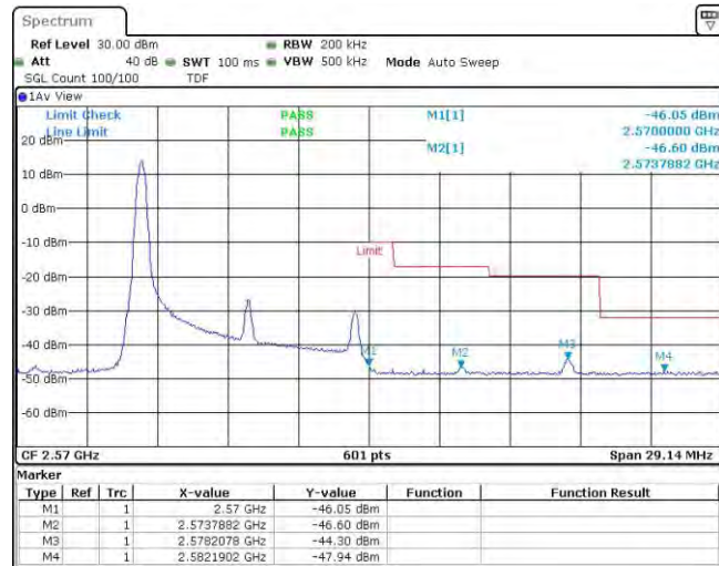
Band7-10MHz-QPSK-21400-1RB#49
