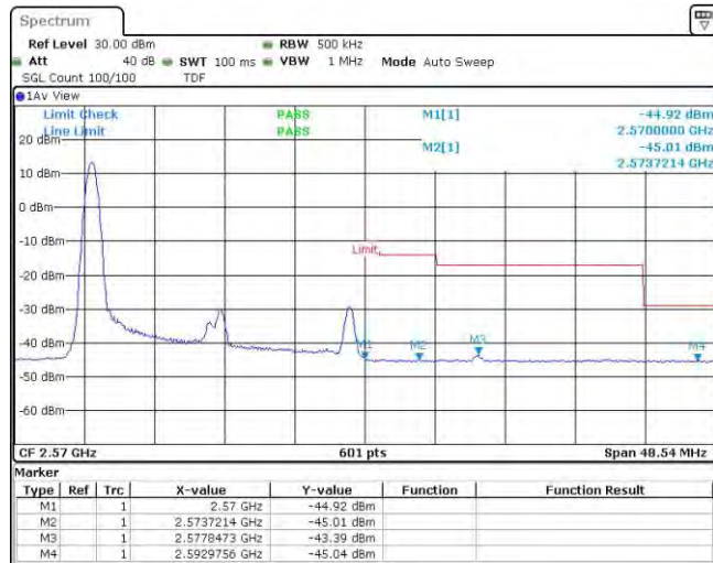
Band7-20MHz-QPSK-21350-1RB#99
