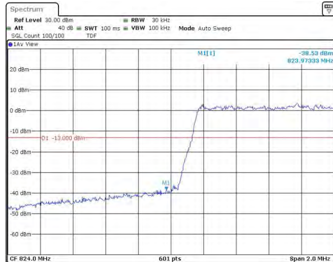
Band5-1.4MHz-16QAM-20643-1RB#0
