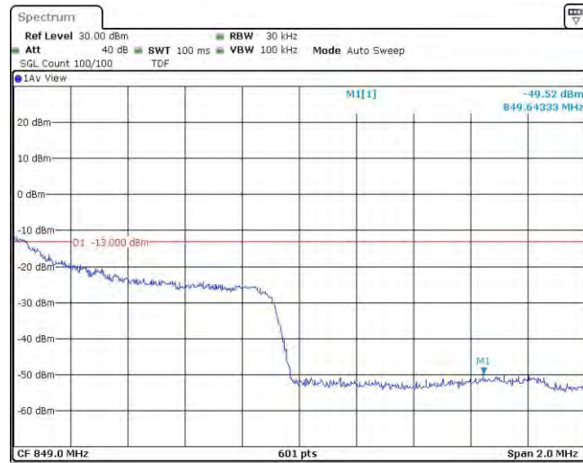
Band5-1.4MHz-QPSK-20643-1RB#5
