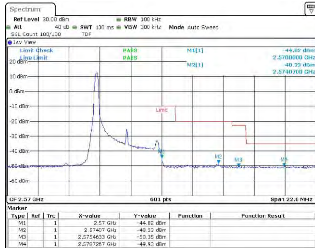
Band7-5MHz-QPSK-21425-1RB#24
