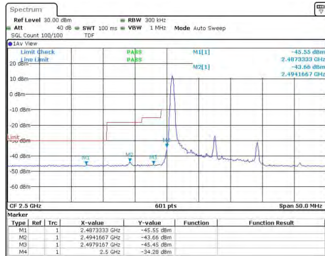
Band7-15MHz-16QAM-20825-1RB#74
