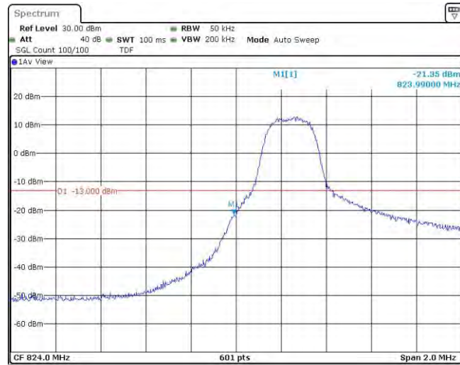
Band5-3MHz-16QAM-20415-1RB#14
