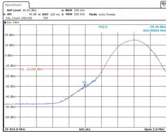
Band5-10MHz-16QAM-20450-1RB#49
