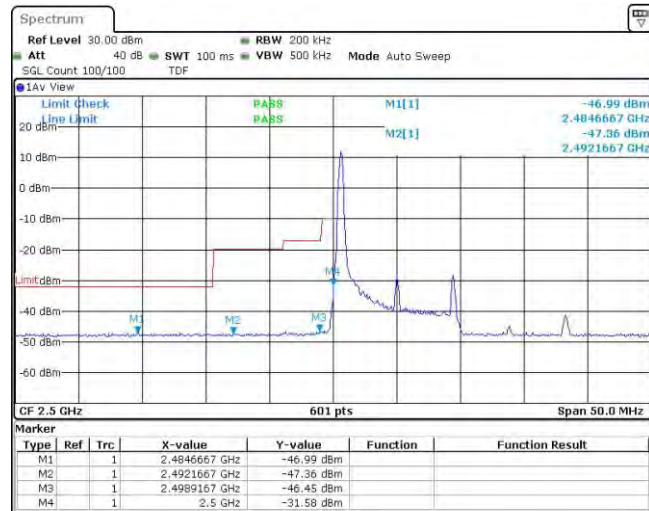
Band7-10MHz-16QAM-20800-1RB#49
