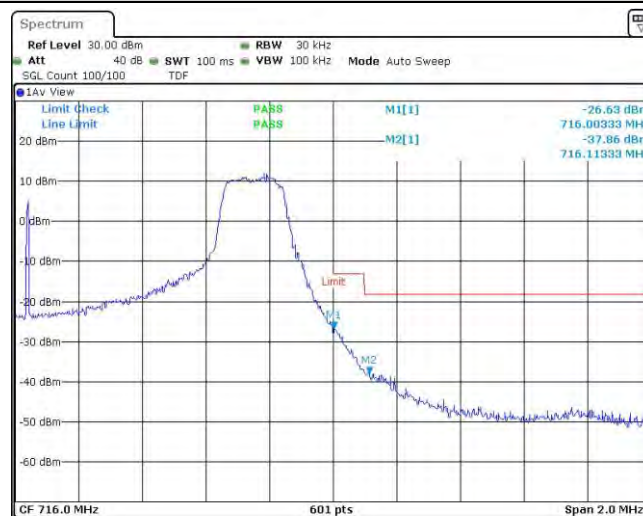
Band12-1.4MHz-QPSK-23173-6RB#0
