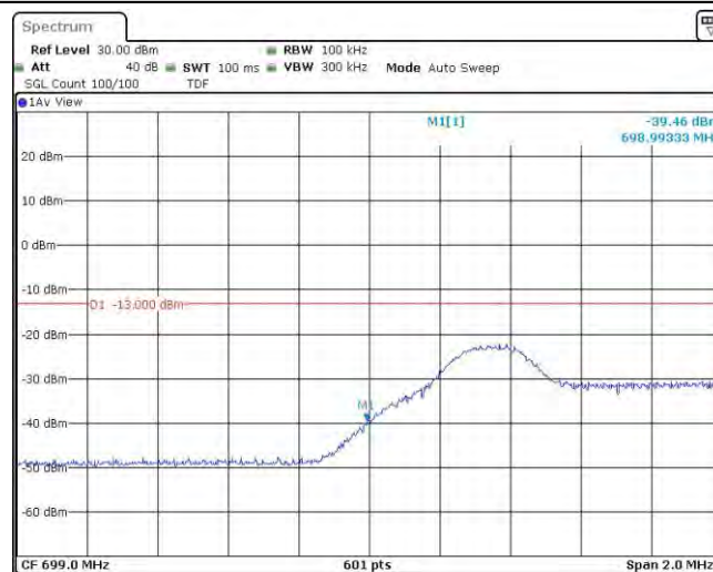
Band12-5MHz-QPSK-23035-25RB#0
