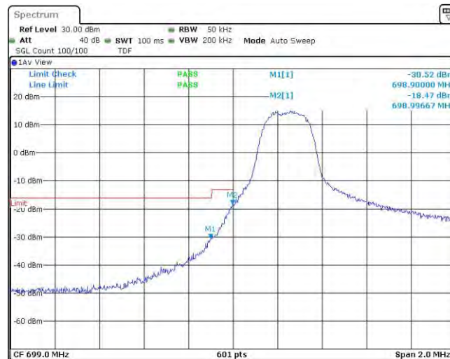
Band12-3MHz-16QAM-23025-1RB#14
