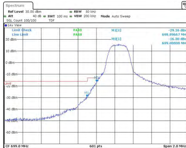
Band12-3MHz-QPSK-23025-1RB#14
