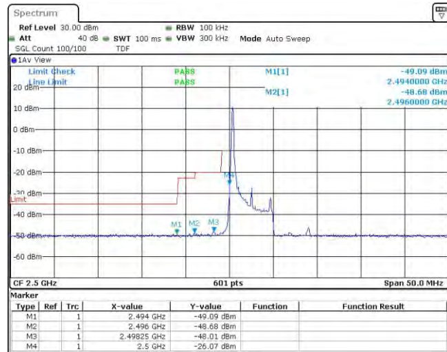
Band7-5MHz-16QAM-20775-1RB#24
