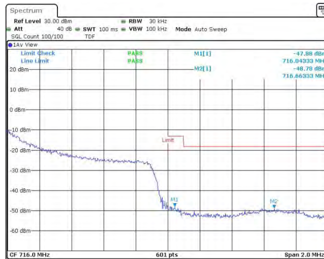
Band12-1.4MHz-QPSK-23173-1RB#5
