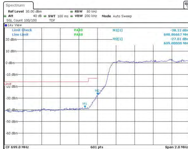
Band12-3MHz-16QAM-23165-1RB#0
