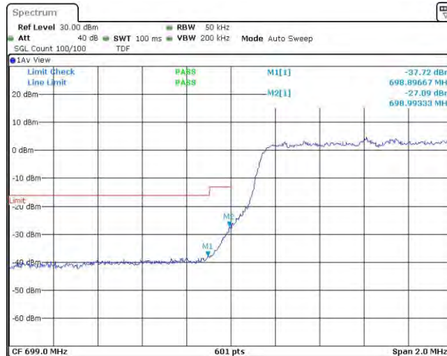
Band12-3MHz-QPSK-23165-1RB#0
