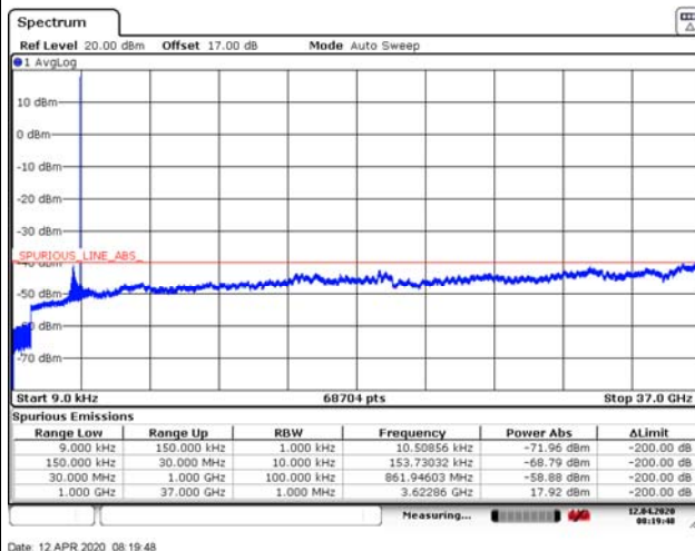
LTE Band 48 5MHz CH Middle 9KHz~37GHz
