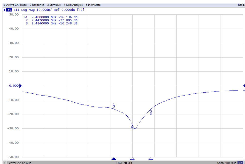
Return Loss
