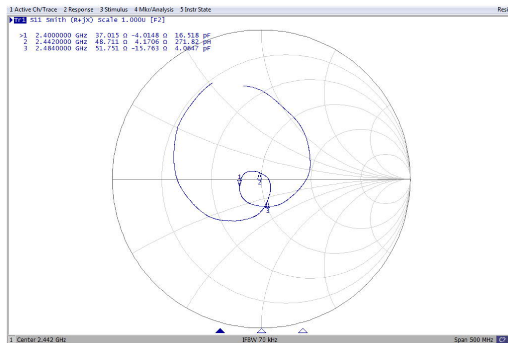
Smith chart
