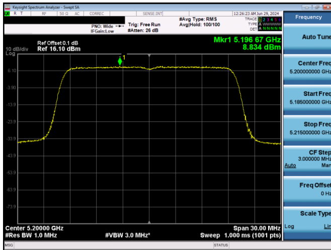
Plot 7-170. PSD Antenna WF5T (20MHz BW 802.11ax(SU) – Ch. 40, MCS2)
