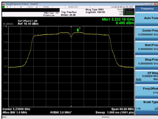
Plot 7-171. PSD Antenna WF5T (40MHz BW 802.11n – Ch. 46, MCS2)
