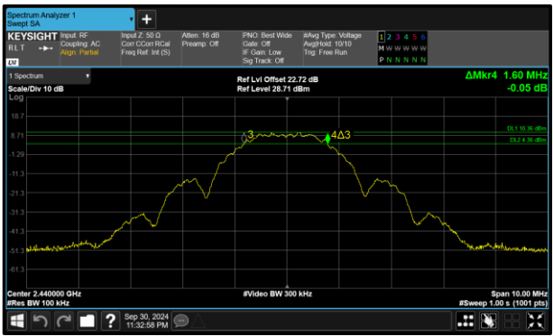
Figure 20 - Core 1 (B) 2440 MHz (CH18) 6 dB Bandwidth
