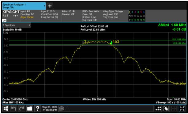
Figure 34 - Core 0 (A) 2475 MHz (CH25) 6 dB Bandwidth
