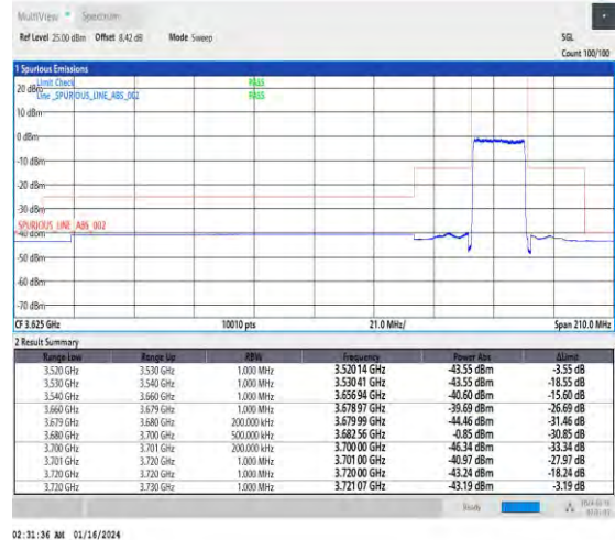
1-N48-30-20-H-3-DFT-PI2BPSK-Outer_Full-50@0-Ant4-1--PASS-see graph
