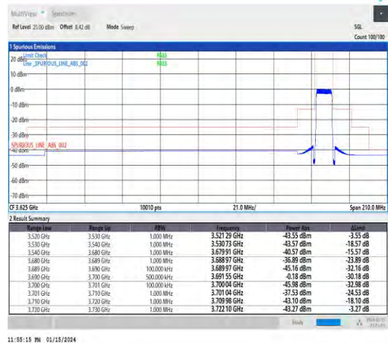
1-N48-30-10-H-6-CP-QPSK-Outer_Full-24@0-Ant4-1--PASS-see graph
