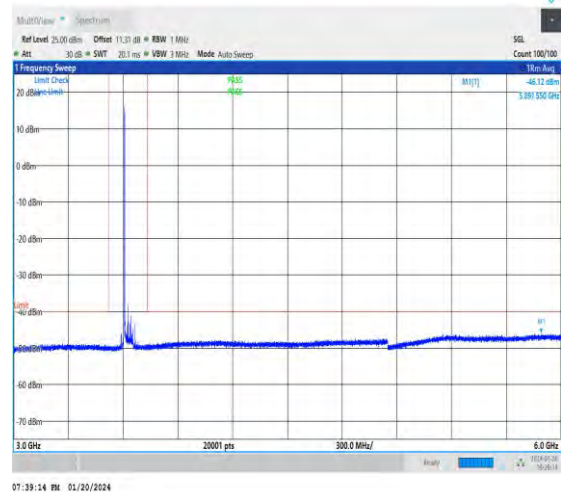
NTNV_N48_30_40_M_TID1_NS_01_3000_6000_#1
