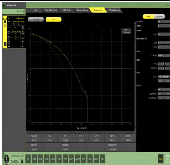
1-N48-30-40-M-12-DFT-256QAM-Outer_Full-100@0
