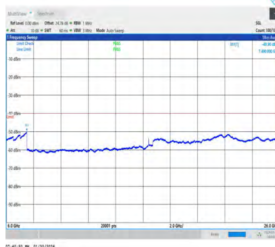
NTNV_N48_30_40_H_TID1_NS_01_6000_26000_#1
