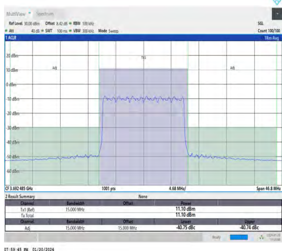
NTNV_N48_30_15_H_TID16_#1_-15_15
