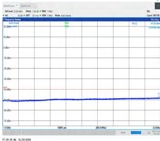
NTNV_N48_30_40_M_TID1_NS_01_1000_3000_#1
