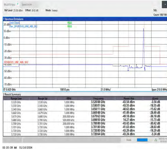
1-N48-30-20-H-2-DFT-PI2BPSK-Edge_1RB_Right-1@50-Ant4-1--PASS-see graph
