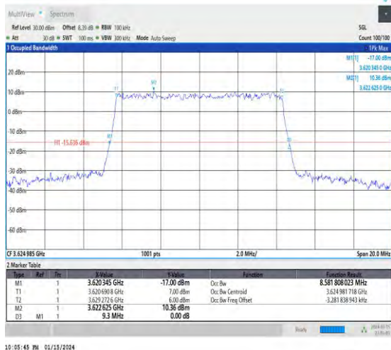
1-N48-30-10-M-3-DFT-16QAM-Outer_Full-24@0-Ant 4-8.582-9.300-≤10-PASS
