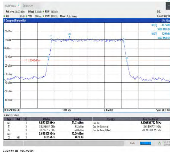
1-N48-30-10-M-2-DFT-PI2BPSK-Outer_Full-24@0-Ant4 -8.607-9.320-≤10-PASS
