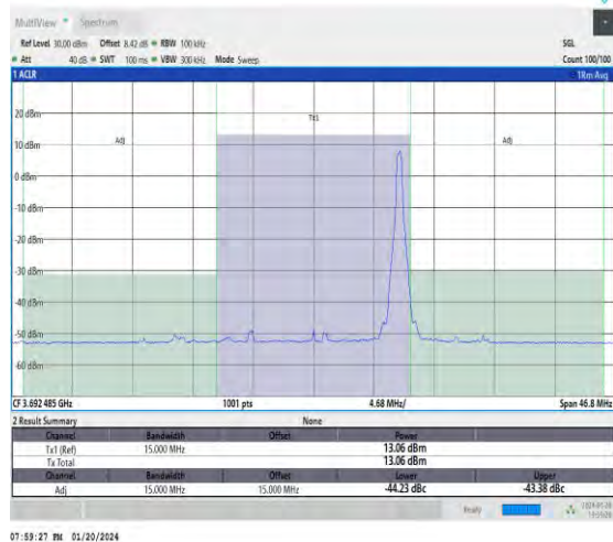
NTNV_N48_30_15_H_TID3_#1_-15_15
