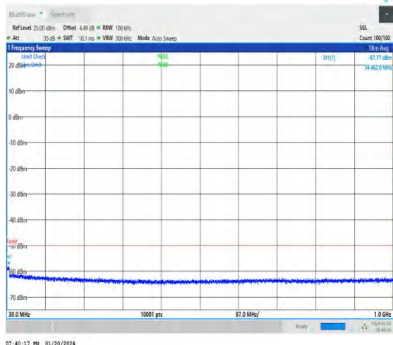
NTNV_N48_30_40_H_TID1_NS_01_30_1000_#1
