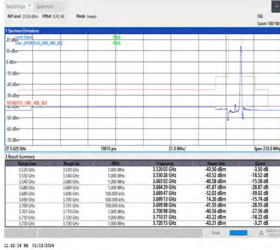
1-N48-30-10-H-2-DFT-PI2BPSK-Edge_1RB_Right-1@23-Ant4-1--PASS-see graph
