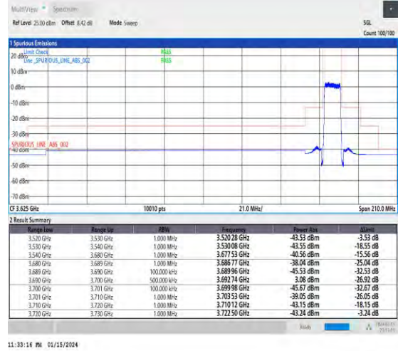
1-N48-30-10-H-3-DFT-PI2BPSK-Outer_Full-24@0-Ant4-1--PASS-see graph
