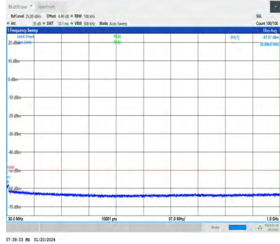
NTNV_N48_30_40_M_TID1_NS_01_30_1000_#1
