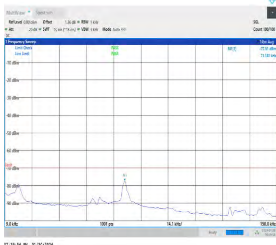
NTNV_N48_30_40_H_TID1_NS_01_0.009_0.15_#1
