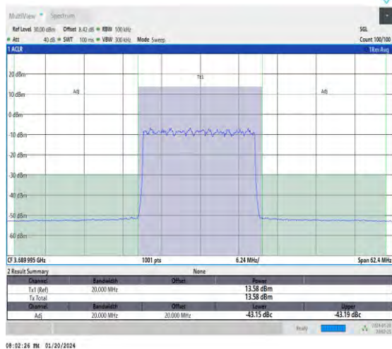
NTNV_N48_30_20_H_TID1_#1_-20_20
