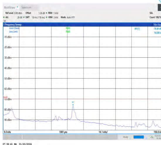
NTVN_N48_30_40_M_TID1_NS_01_0.009_0.15_#1
