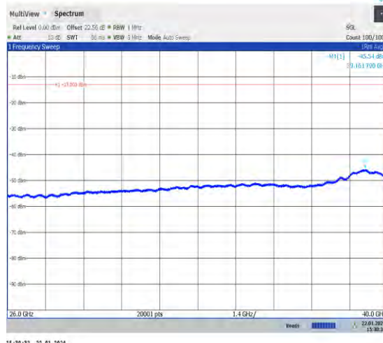
NTNV_N48_30_40_M_TID1_NS_01_26000_40000_#1
