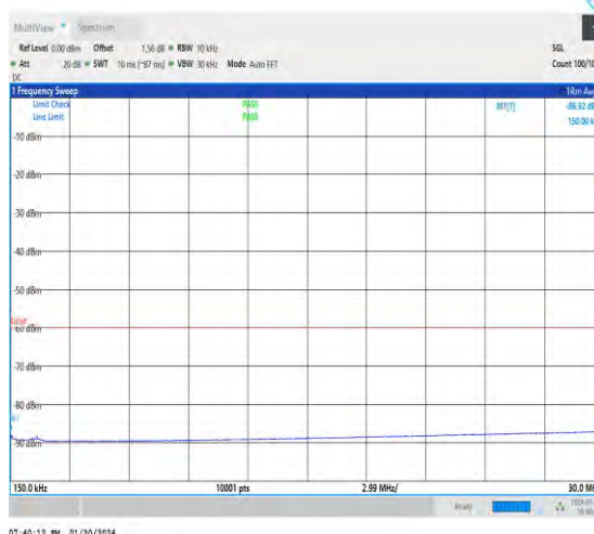
NTNV_N48_30_40_H_TID1_NS_01_0.15_30_#1
