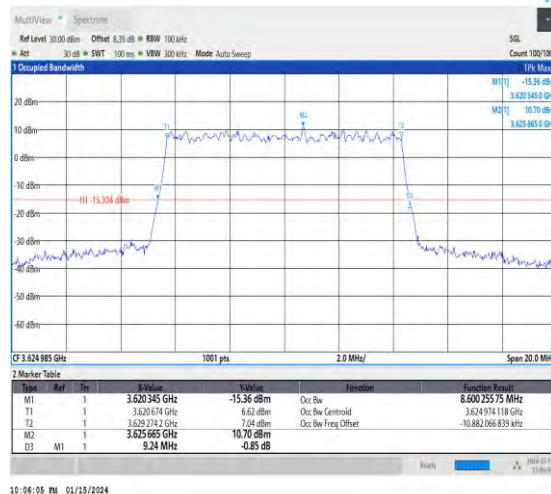
1-N48-30-10-M-4-DFT-64QAM-Outer_Full-24@0-Ant 4-8.6-9.240-≤10-PASS
