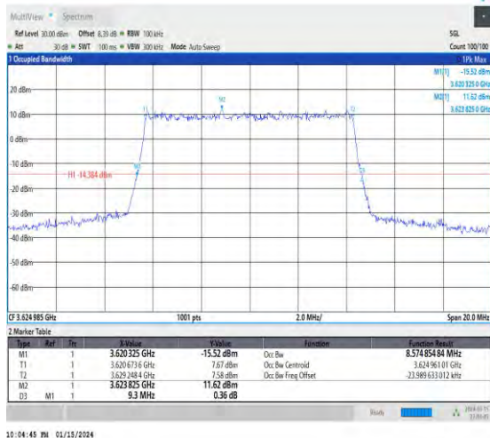
1-N48-30-10-M-1-DFT-QPSK-Outer_Full-24@0-Ant4 -8.575-9.300-≤10-PASS
