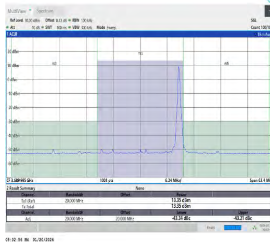
NTNV_N48_30_20_H_TID3_#1_-20_20
