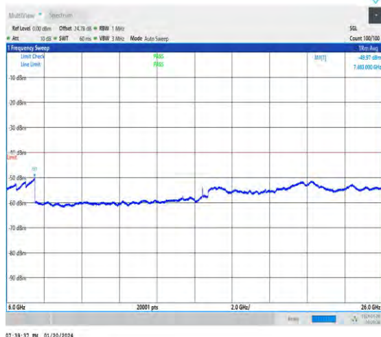
NTNV_N48_30_40_M_TID1_NS_01_6000_26000_#1
