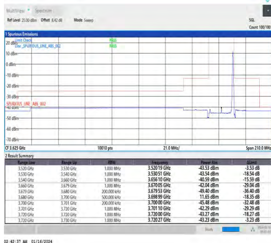
1-N48-30-20-H-5-CP-QPSK-Edge_1RB_Right-1@50-Ant4-1--PASS-see graph
