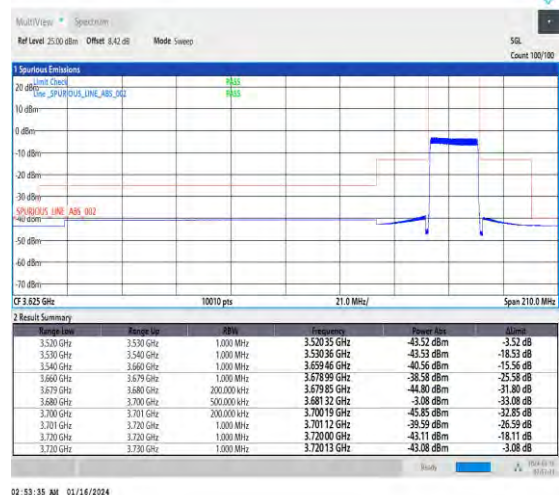
1-N48-30-20-H-6-CP-QPSK-Outer_Full-51@0-Ant4-1--PASS-see graph
