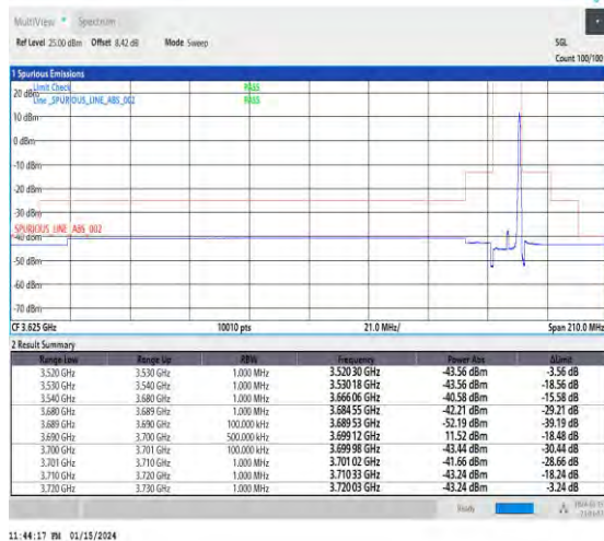
1-N48-30-10-H-5-CP-QPSK-Edge_1RB_Right-1@23-Ant4-1--PASS-see graph
