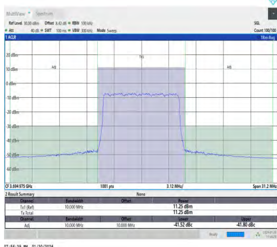
NTNV_N48_30_10_H_TID16_#1_-10_10
