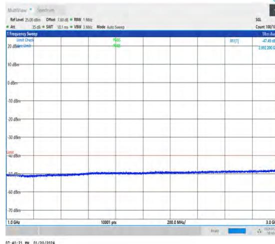
NTNV_N48_30_40_H_TID1_NS_01_1000_3000_#1
