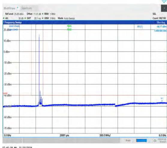
NTNV_N48_30_40_H_TID1_NS_01_3000_6000_#1
