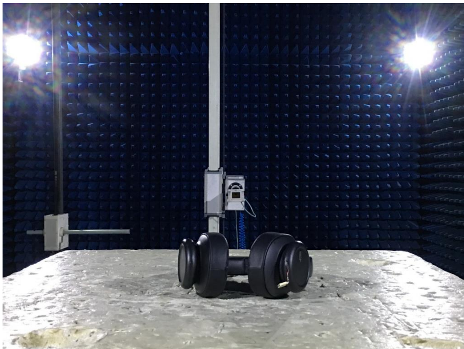
Photograph : Set-up for Radiated Spurious Emission, 18GHz - 26.5GHz
