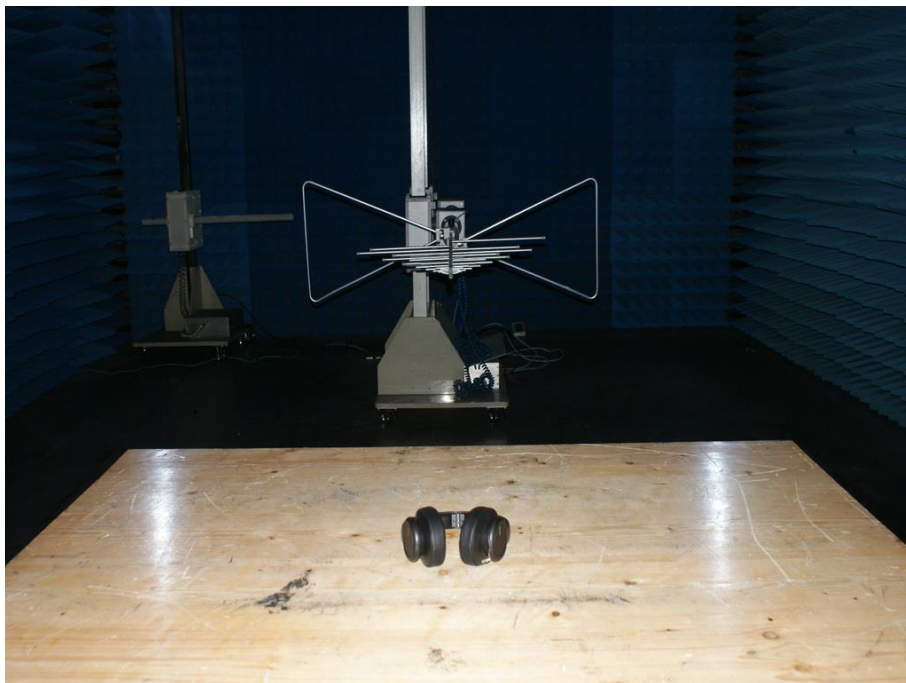
Photograph : Set-up for Radiated Spurious Emission, 30MHz - 1GHz
