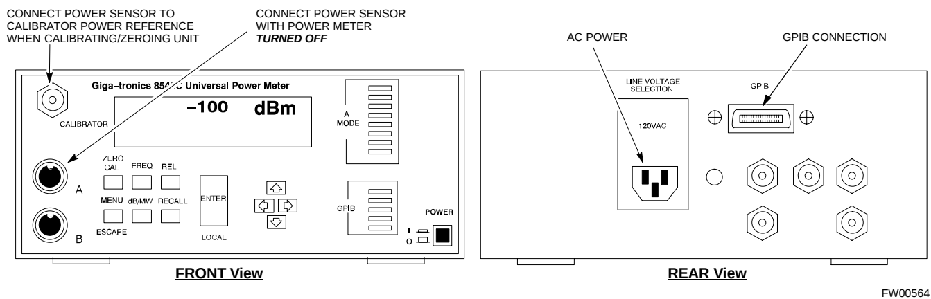
Figure F-20: Gigatronics 8541C Power Meter Detail
