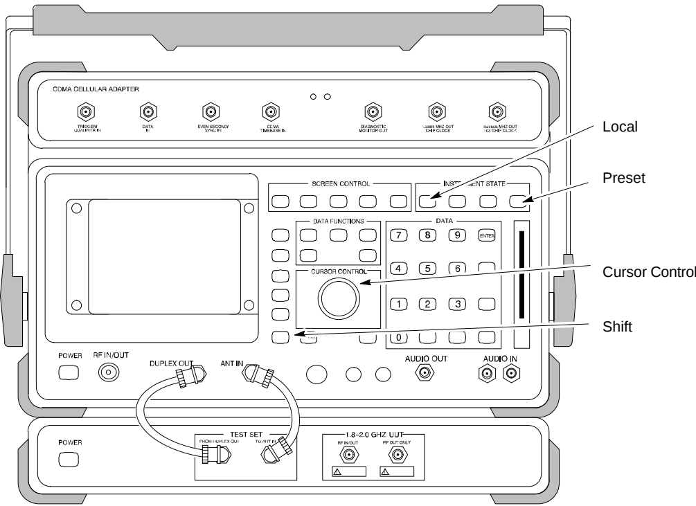
Figure F-6: HP 8921A and HP 83236A/B
