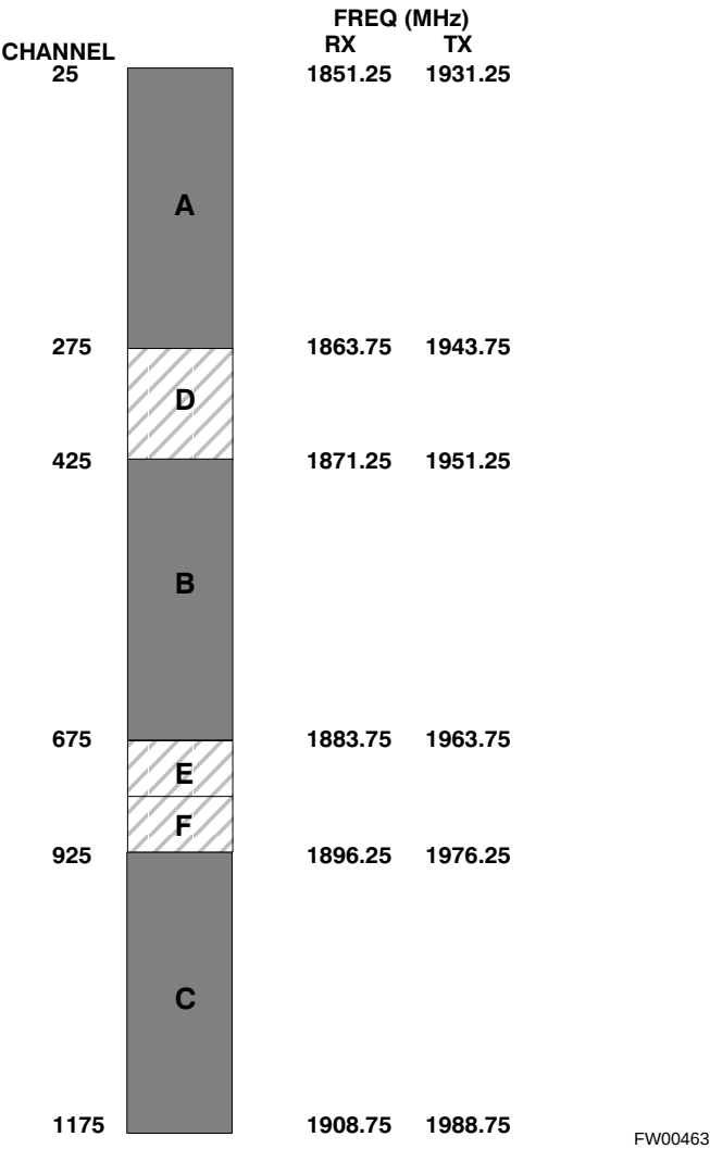
Figure E-1: North America PCS Frequency Spectrum (CDMA Allocation)
