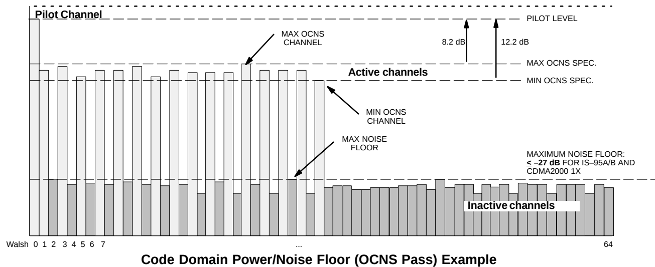
Figure 4-3: Code Domain Analyzer CD Power/Noise Floor Display Examples
