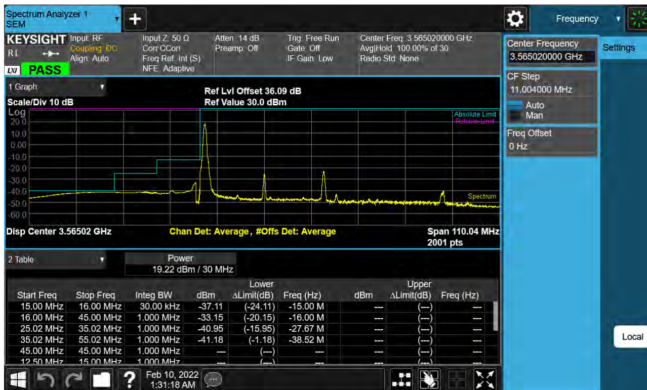
Sub6 n48. 30 M_BandEdge(Lower)_Low_ 3565.02 MHz_BPSK_1RB
