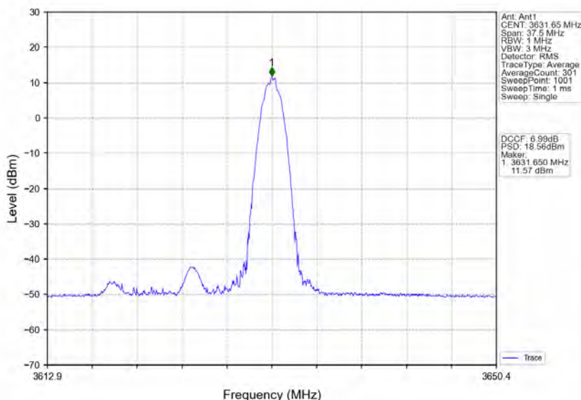
n78d_30kHz_MIMO_NTNV_15MHz_CP-OFDM_16_QAM_3624.99MHz_Edge_1RB_Right
