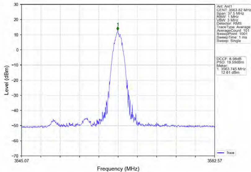
n78d_30kHz_MIMO_NTNV_15MHz_CP-OFDM_QPSK_3557.52MHz_Inner_1RB_Right
