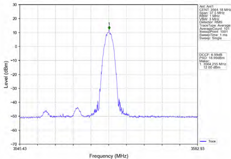
n78d_30kHz_MIMO_NTNV_15MHz_CP-OFDM_16_QAM_3557.52MHz_Edge_1RB_Right
