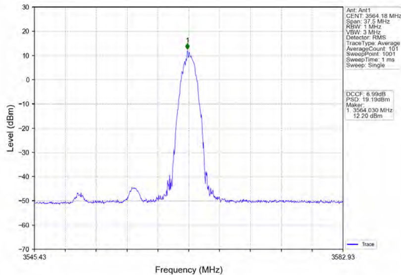
n78d_30kHz_MIMO_NTNV_15MHz_CP-OFDM 64 QAM_3557.52MHz_Edge_1RB_Right
