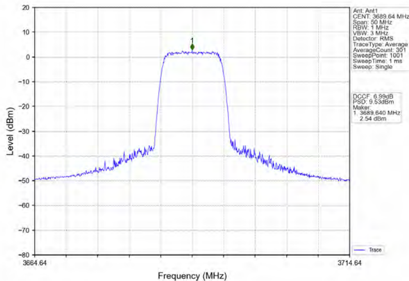
n78d_30kHz_MIMO_NTNV_20MHz_CP-OFDM_64_QAM_3690MHz_Inner_Full
