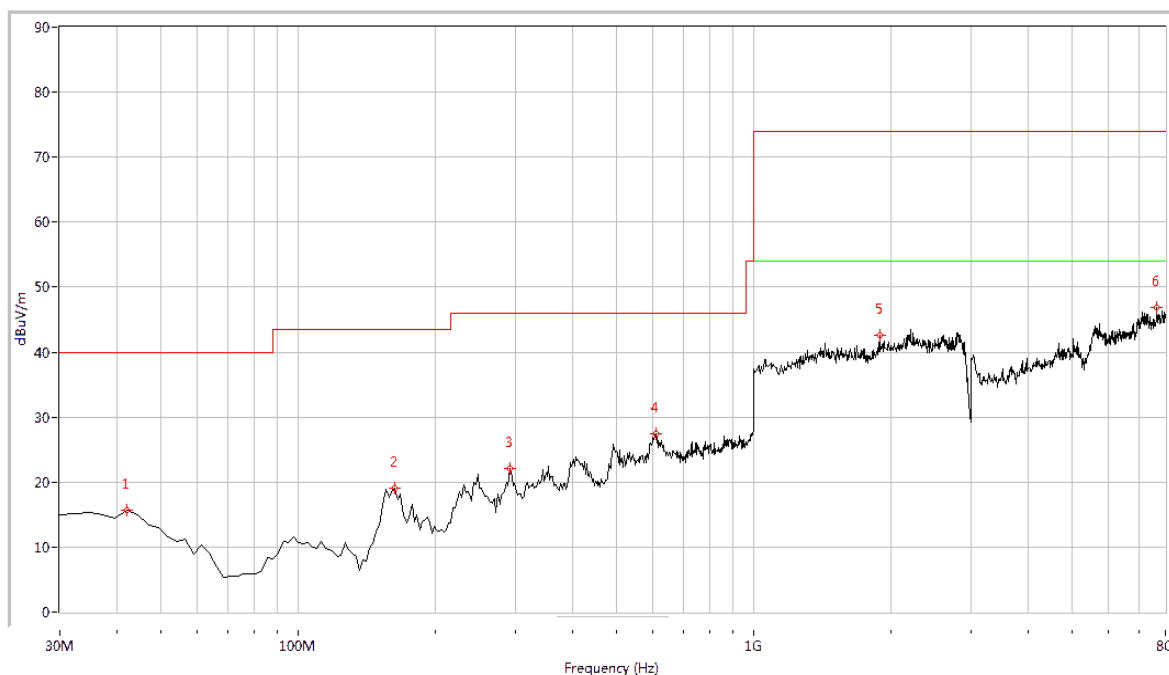
(Plot B: 30MHz – 8GHz, Test Antenna Horizontal)
