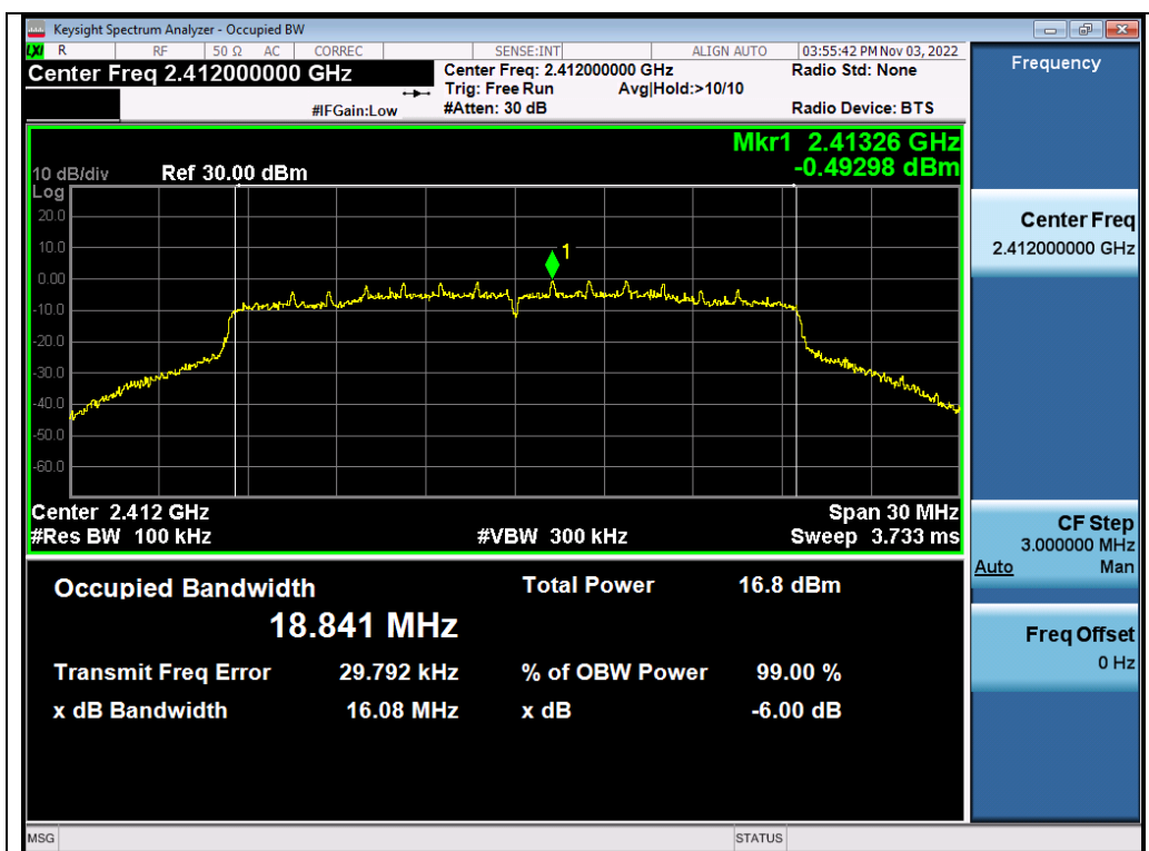
Test_Graph_802.11ax20_ANT1_2412_MCS0_DTSBW
