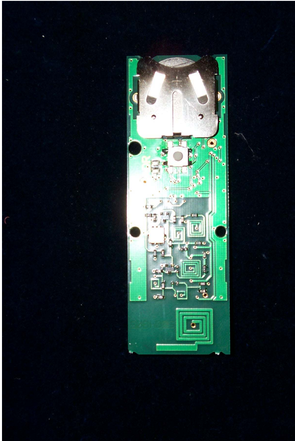
Figure 6.5 Foil Side
