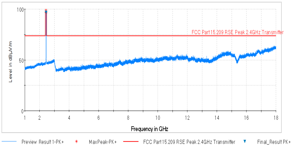
Plot 6-38. Radiated Spurious Plot above 1GHz (802.11b – Ch. 6, Ant. Pol. V)
