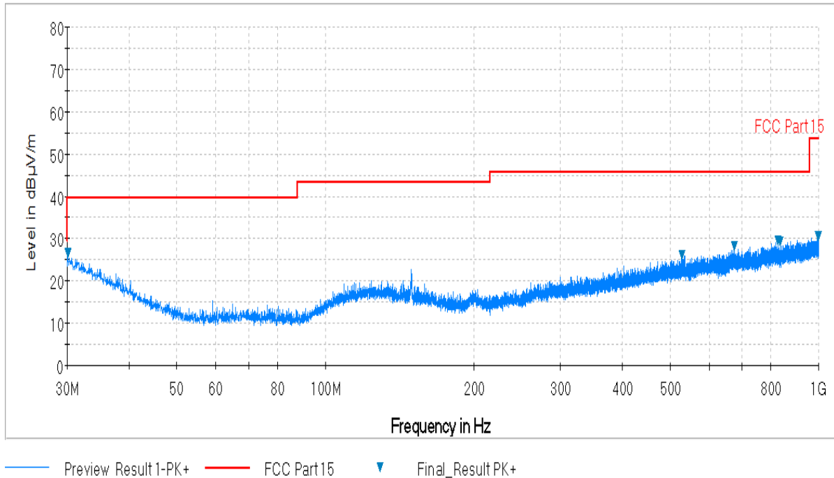
Plot 6-51. Radiated Spurious Plot below 1GHz (Pol. H)
