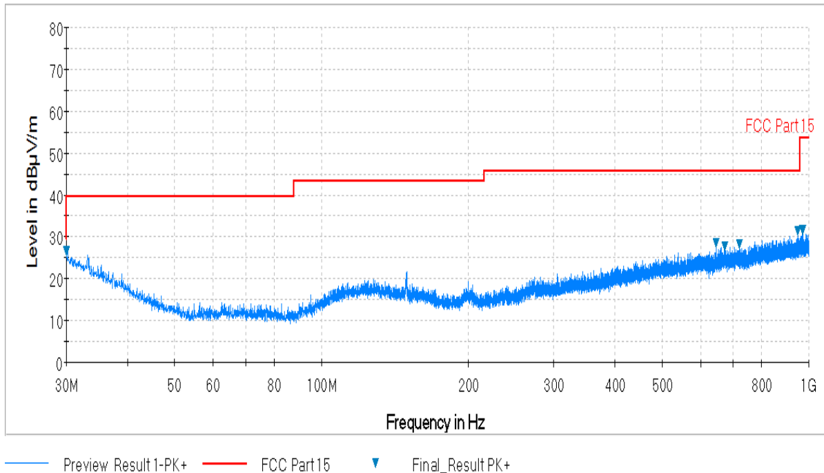
Plot 6-52. Radiated Spurious Plot below 1GHz (Pol. V)
