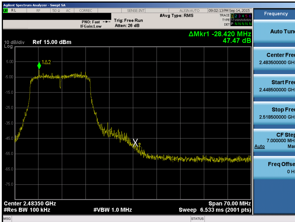
Plot 6-28. Band Edge Plot (802.11n (2.4GHz) – Ch. 11)
