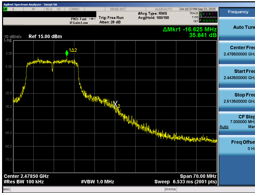
Plot 6-27. Band Edge Plot (802.11n (2.4GHz) – Ch. 10)
