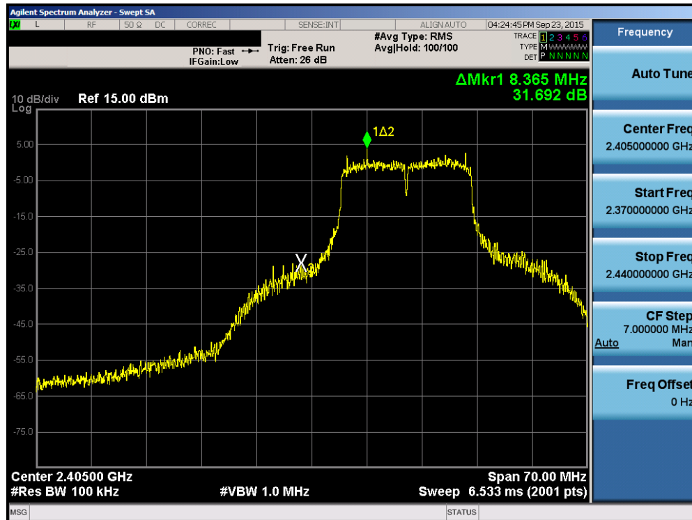
Plot 6-22. Band Edge Plot (802.11g— Ch. 2)
