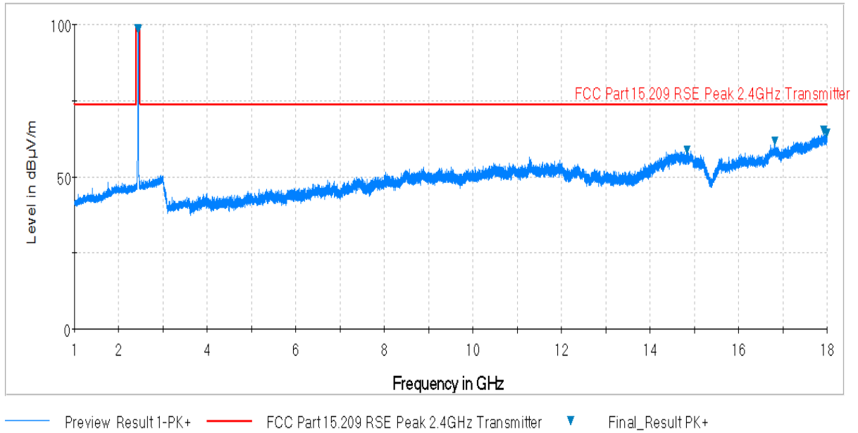
Plot 6-37. Radiated Spurious Plot above 1GHz (802.11b – Ch. 6, Ant. Pol. H)
