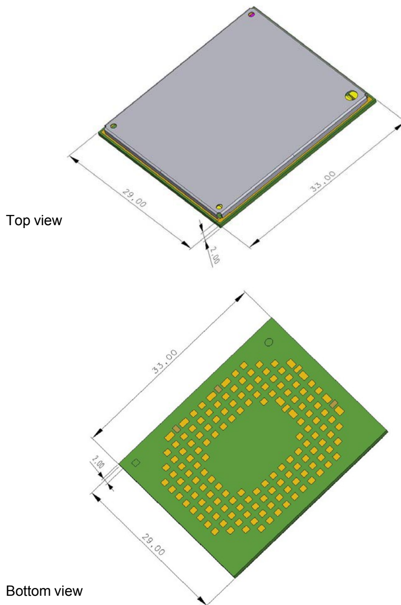
Figure 5: PDS6 – top and bottom view
