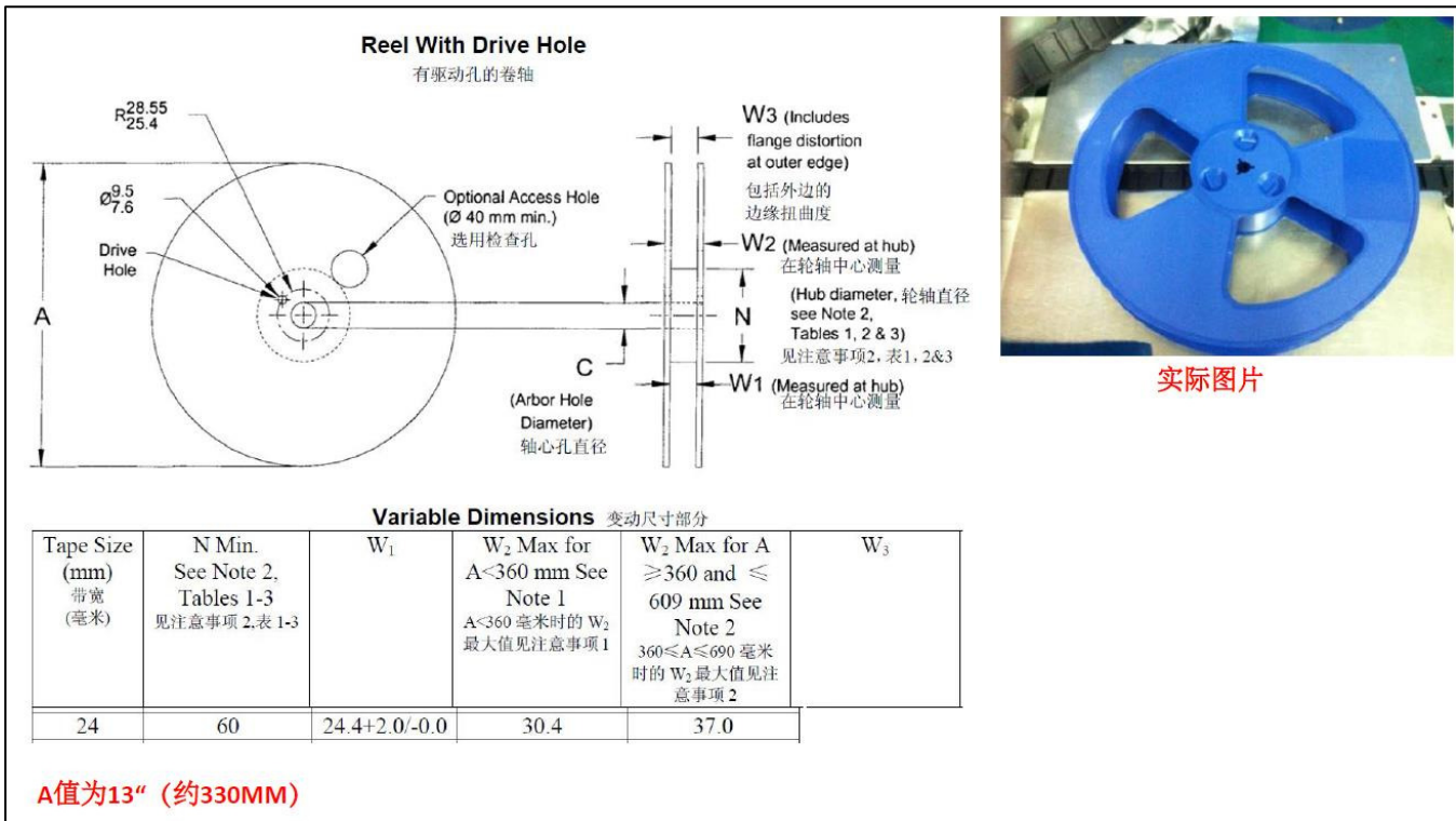
Figure 12: Reel specifications
