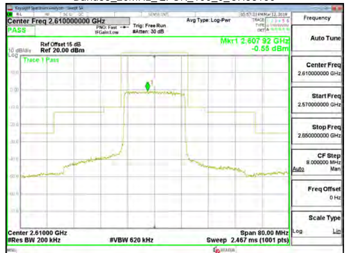
Band38_20MHz_QPSK_100_0_CH38150
