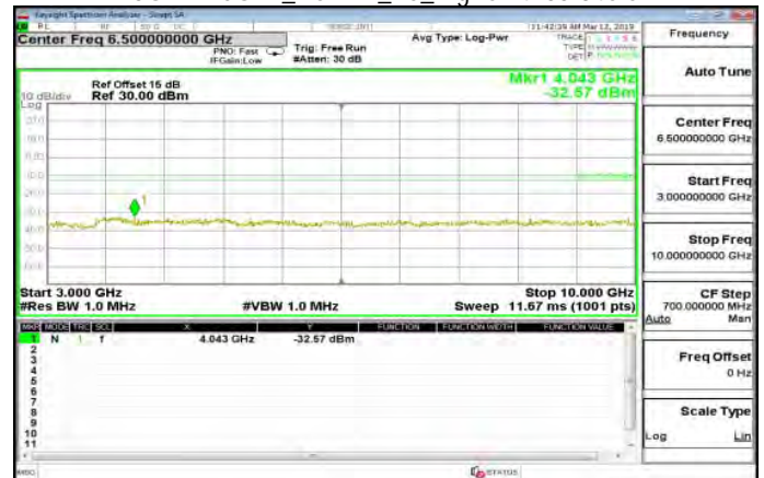
3GHz~10GHz_HSDPA_B5_HighCH4233-846.6
