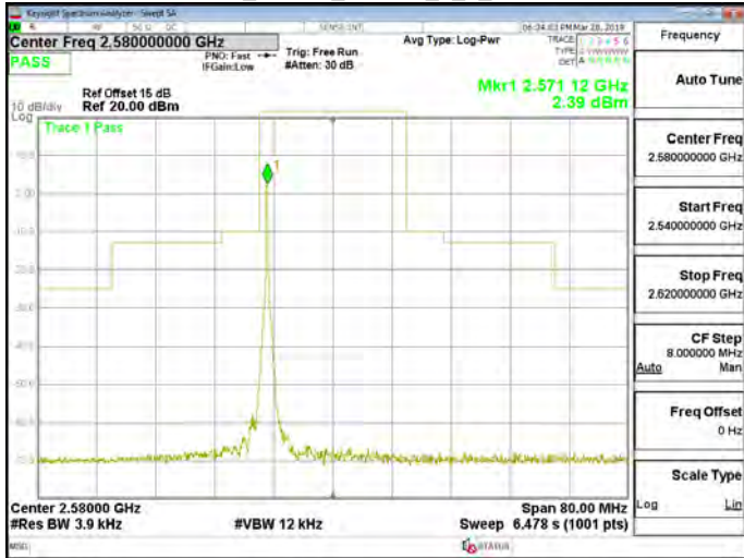
Band38_20MHz_16QAM_1_0_CH38000
