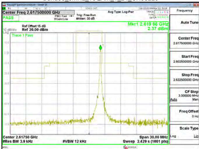
Band38_5MHz_16QAM_1_24_CH38225
