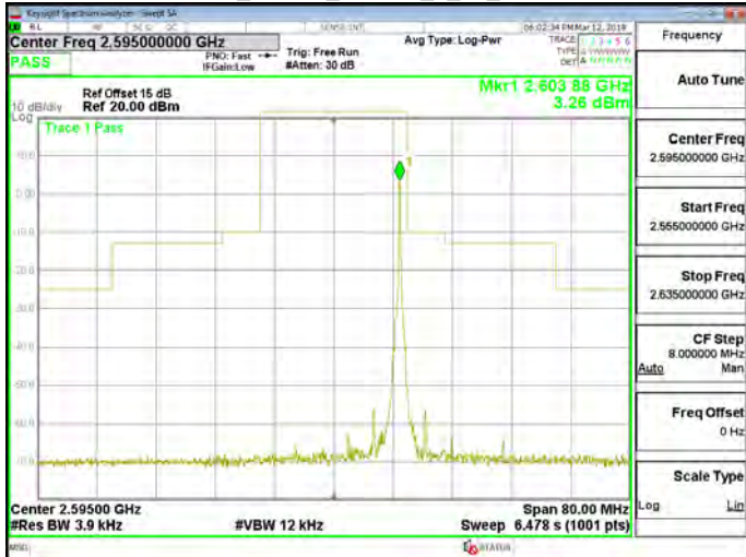
Band38_20MHz_64QAM_1_99_CH38150
