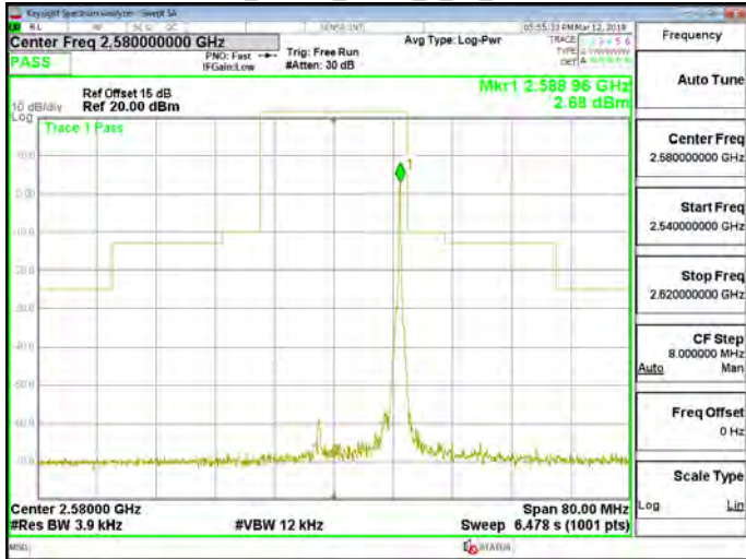
Band38_20MHz_QPSK_1_99_CH38000
