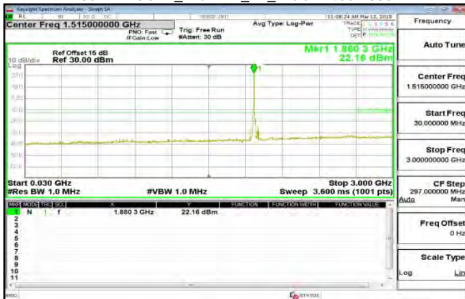
30MHz~3GHz_WCDMA_B2_MidCH9400-1880
