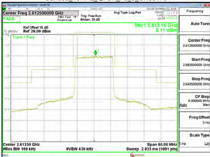
Band38_15MHz_QPSK_75_0_CH38175
