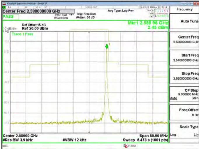
Band38_20MHz_64QAM_1_99_CH38000
