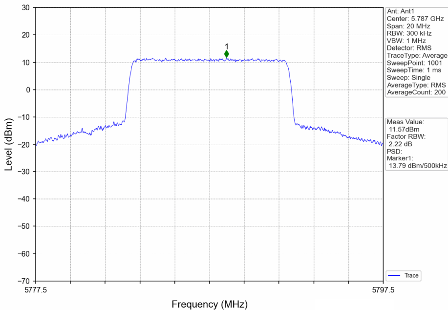
10MHz BW_MCH_5787.5MHz_Ant1_NTNV
