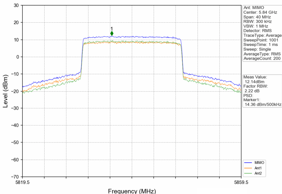
20MHz BW_HCH_5839.5MHz_MIMO_NTNV
