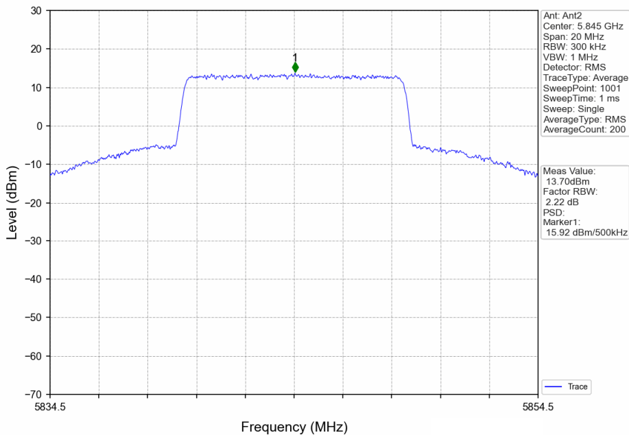
10MHz BW_HCH_5844.5MHz_Ant2_NTNV
