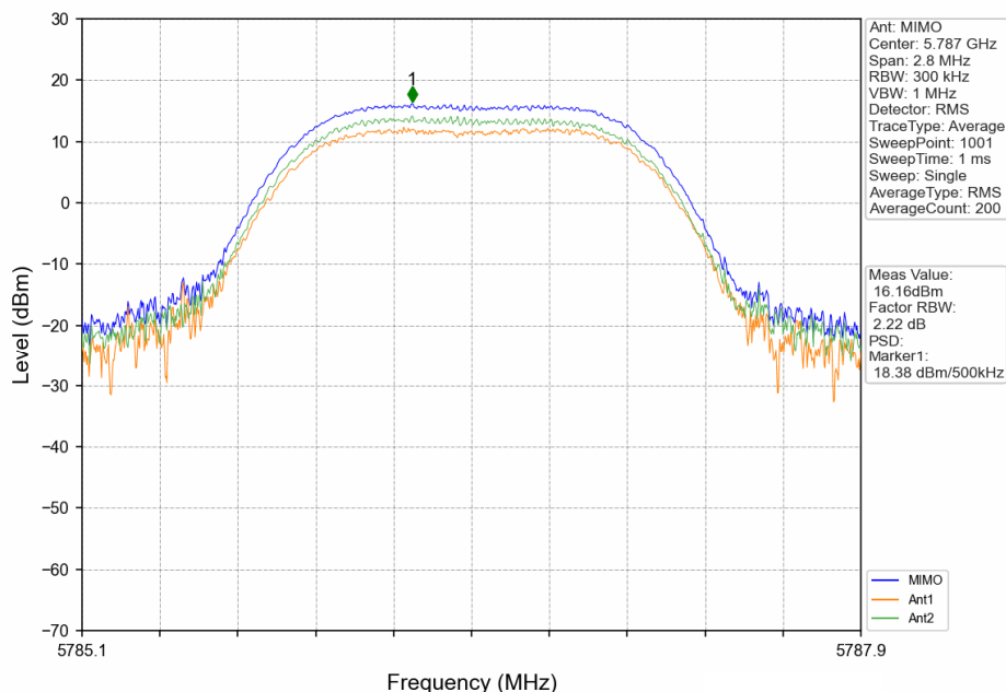
1.4MHz BW_MCH_5786.5MHz_MIMO_NTNV
