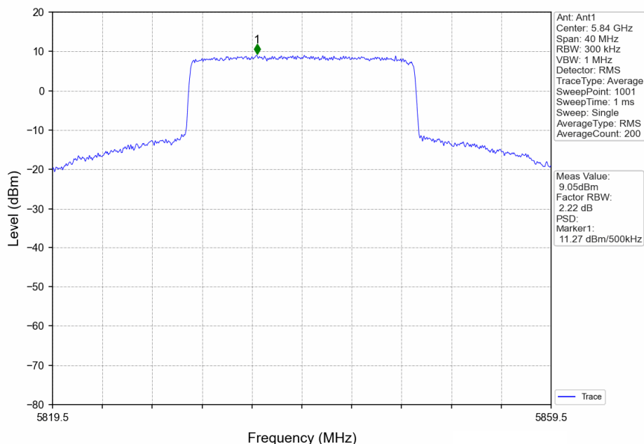
20MHz BW_HCH_5839.5MHz_Ant1_NTNV
