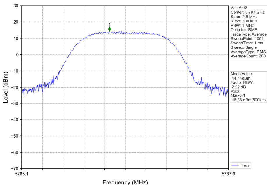
1.4MHz BW_MCH_5786.5MHz_MIMO_NTNV
