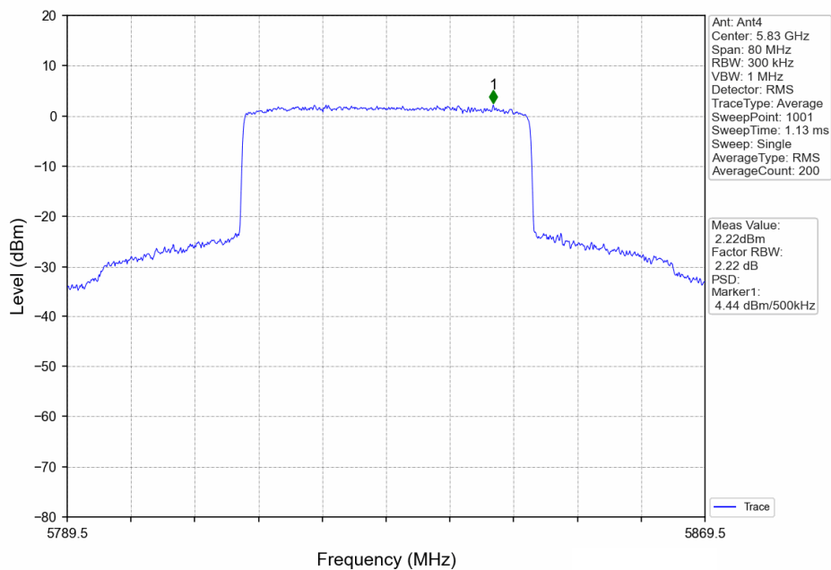
40MHz BW_HCH_5829.5MHz_Ant4_NTNV
