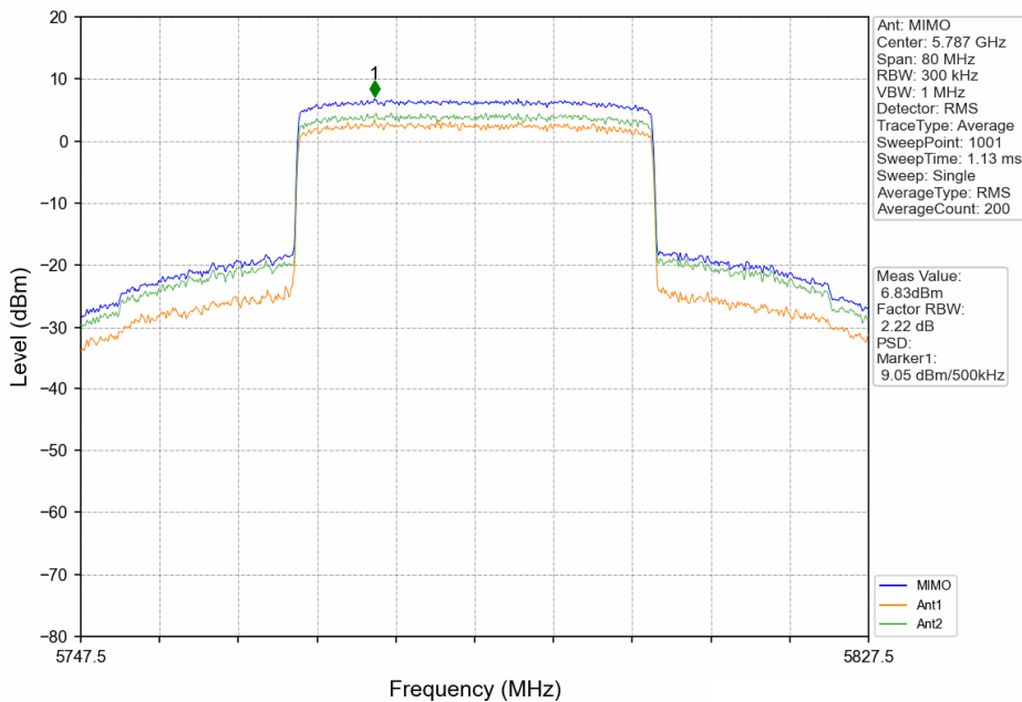
40MHz BW_MCH_5787.5MHz_MIMO_NTNV
