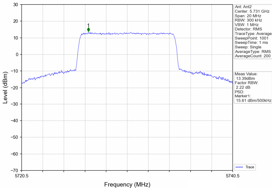
10MHz BW_LCH_5730.5MHz_Ant2_NTNV
