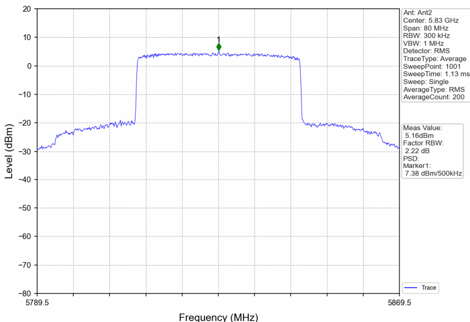
40MHz BW_HCH_5829.5MHz_Ant2_NTNV
