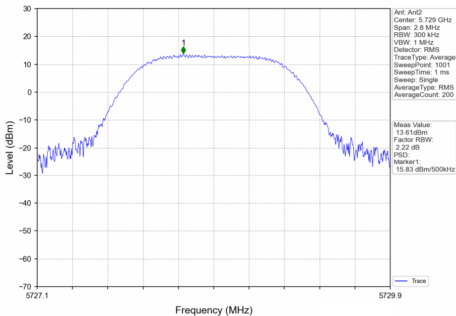
1.4MHz BW_LCH_5728.5MHz_Ant2_NTNV
