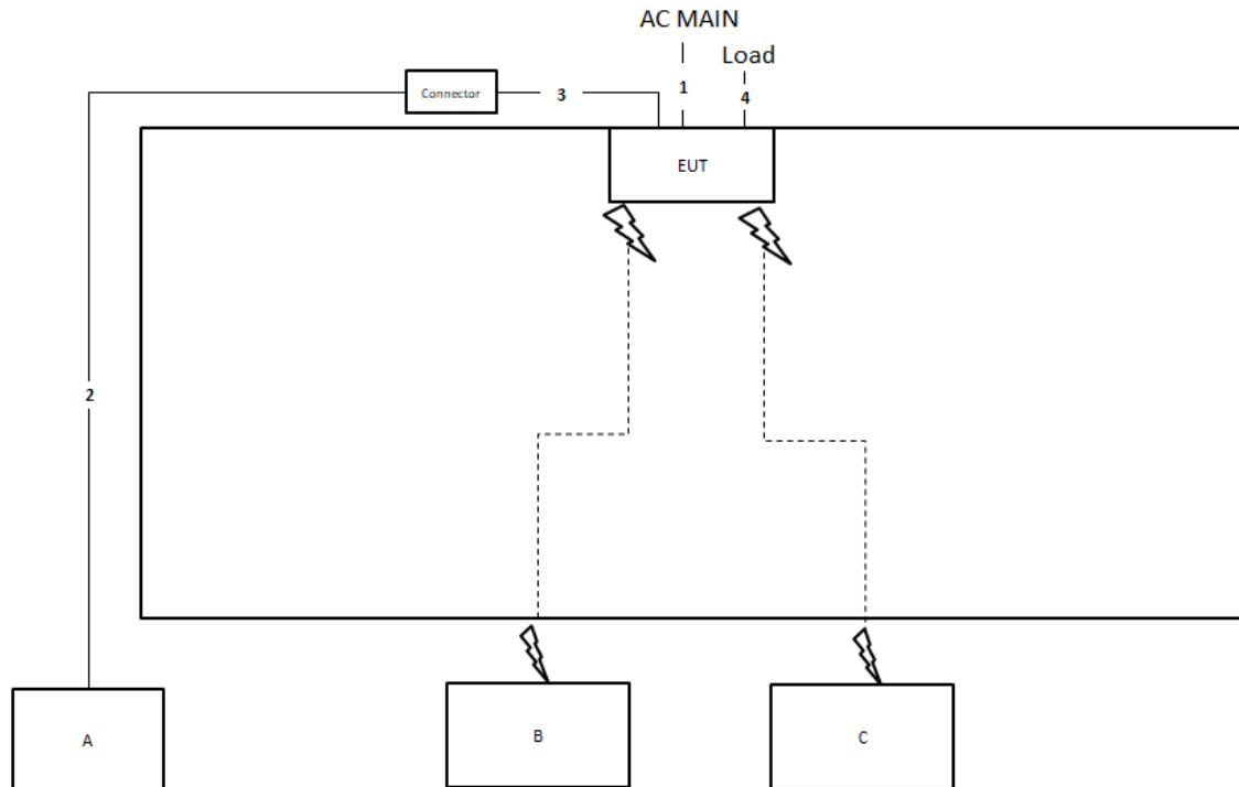
Test Setup Diagram - Radiated Test < 1GHz / Mode 1
