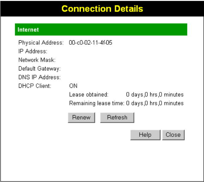
Figure 29: Connection Details - Fixed/Dynamic IP Address
