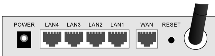
Figure 3: Rear Panel
