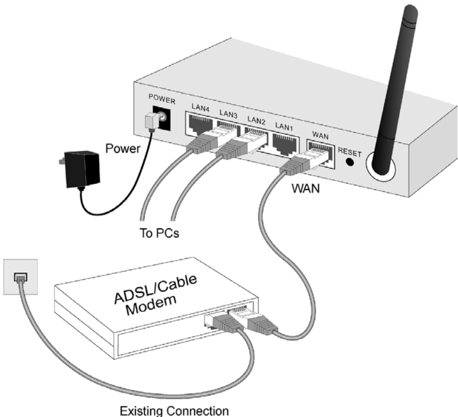
Figure 4: Installation Diagram
