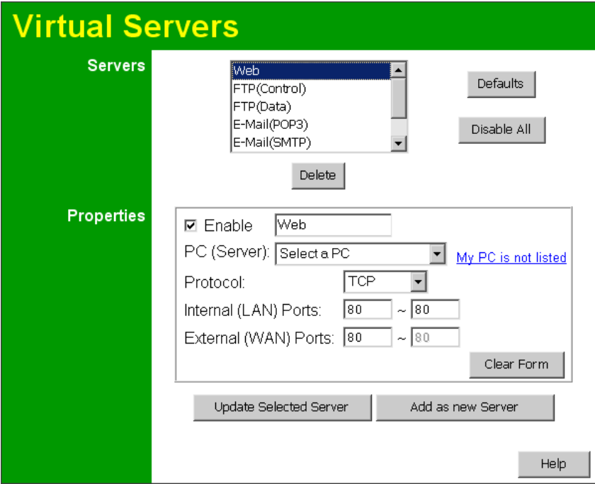
Figure 39: Virtual Servers Screen
