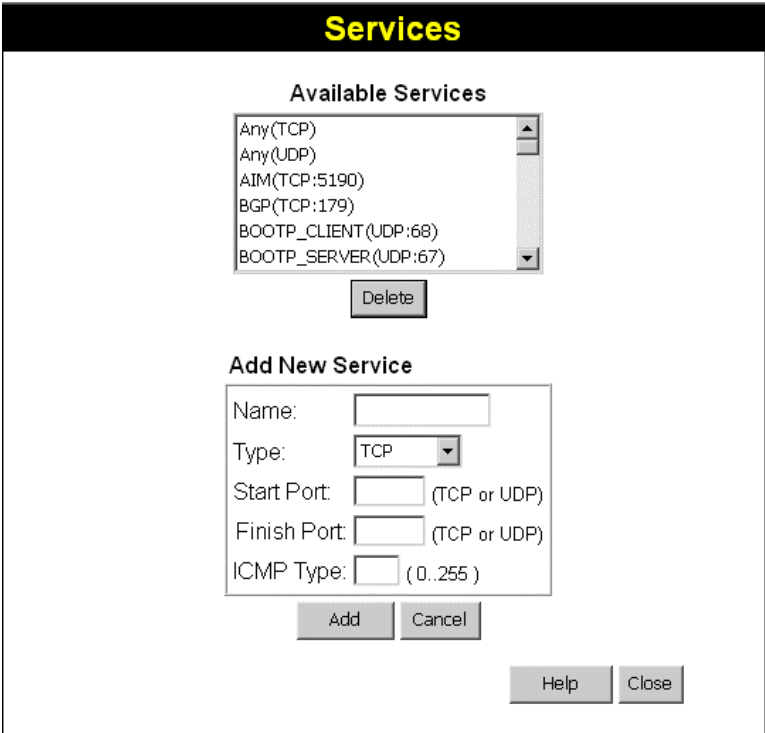
Figure 33: Access Control - Services
