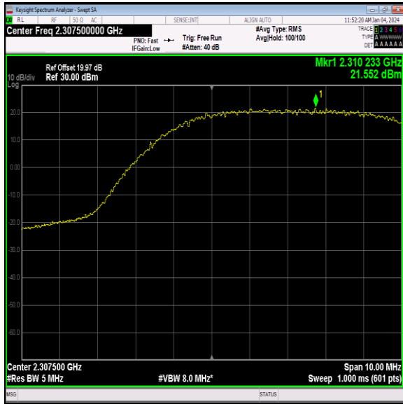
40(2305-2315)-5MHz-64QAM-38725-1RB#24-PASS
