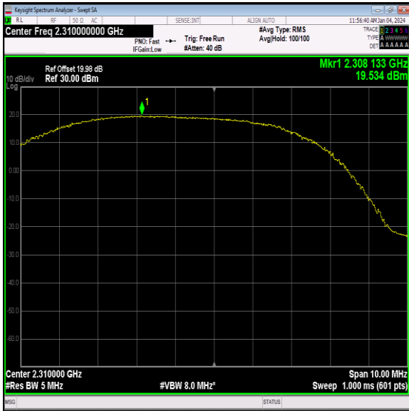
40(2305-2315)-5MHz-64QAM-38750-12RB#11-PASS
