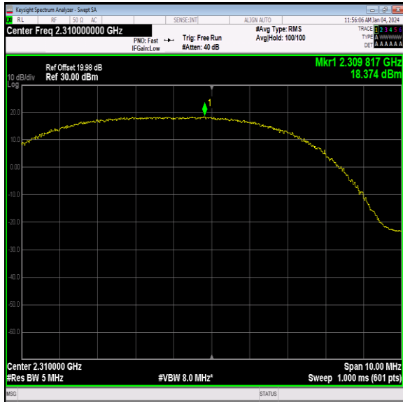
40(2305-2315)-5MHz-16QAM-38750-12RB#6-PASS
