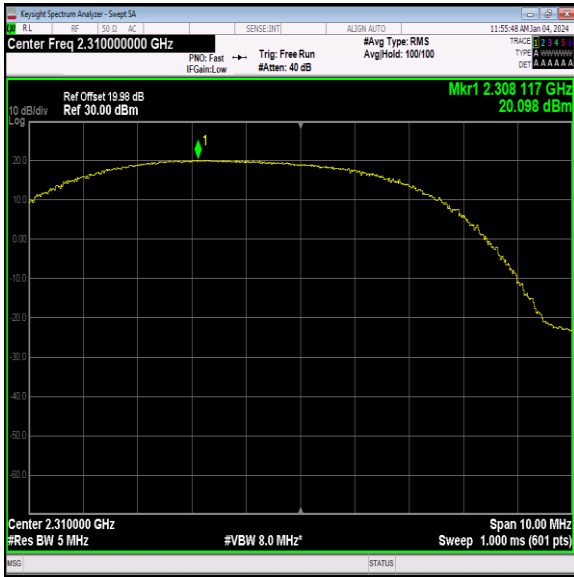
40(2305-2315)-5MHz-64QAM-38750-12RB#0-PASS
