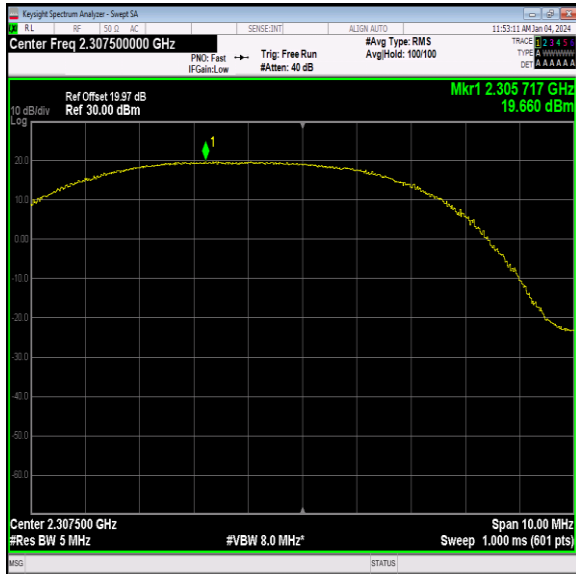
40(2305-2315)-5MHz-64QAM-38725-12RB#6-PASS
