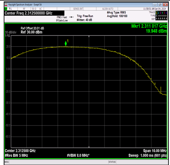
40(2305-2315)-5MHz-64QAM-38775-12RB#0-PASS
