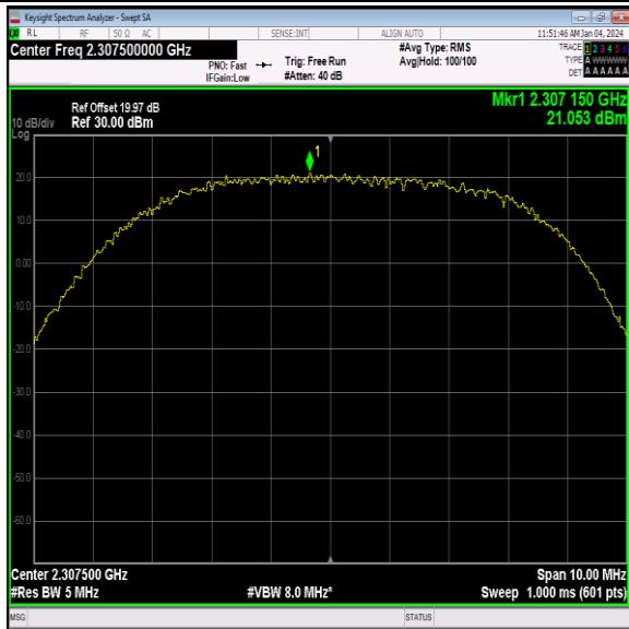
40(2305-2315)-5MHz-16QAM-38725-1RB#12-PASS
