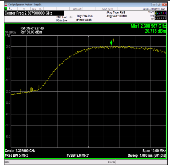
40(2305-2315)-5MHz-16QAM-38725-1RB#24-PASS
