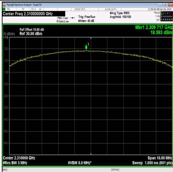
40(2305-2315)-5MHz-16QAM-38750-25RB#0-PASS
