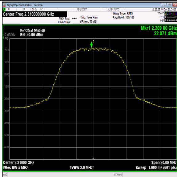
40(2305-2315)-10MHz-64QAM-38750-1RB#24-PASS
