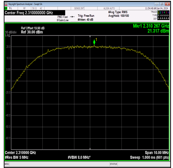
40(2305-2315)-5MHz-16QAM-38750-1RB#12-PASS
