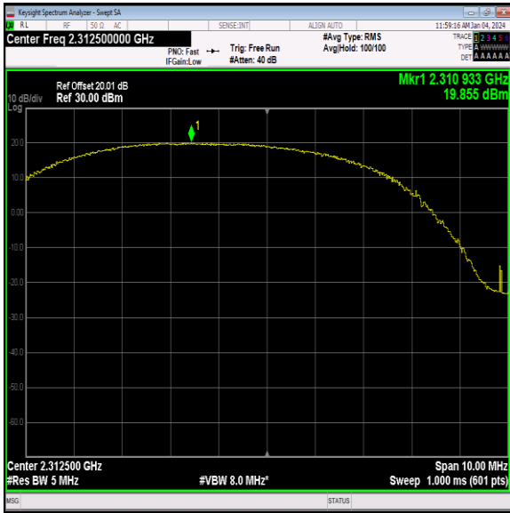
40(2305-2315)-5MHz-64QAM-38775-12RB#6-PASS
