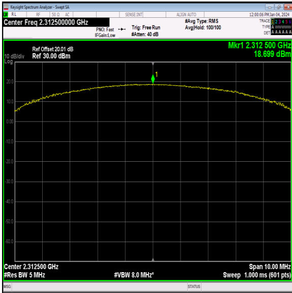
40(2305-2315)-5MHz-64QAM-38775-25RB#0-PASS
