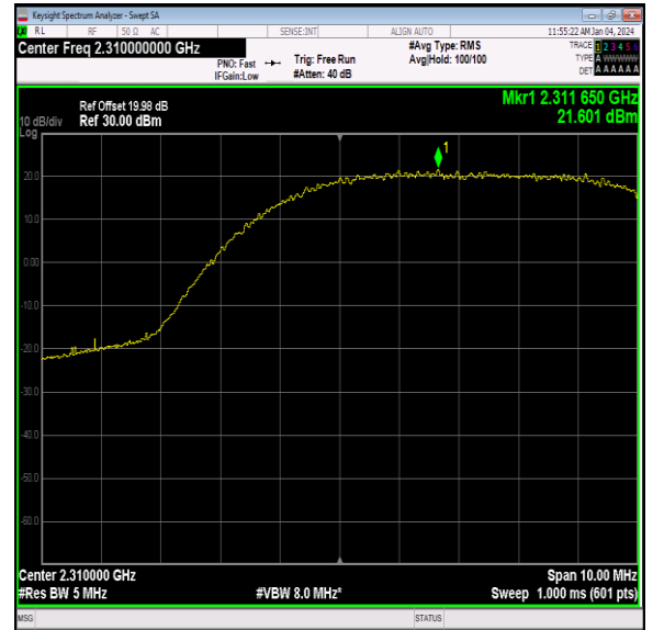
40(2305-2315)-5MHz-64QAM-38750-1RB#24-PASS
