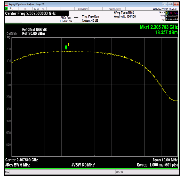
40(2305-2315)-5MHz-16QAM-38725-12RB#6-PASS
