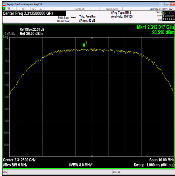
40(2305-2315)-5MHz-16QAM-38775-1RB#12-PASS
