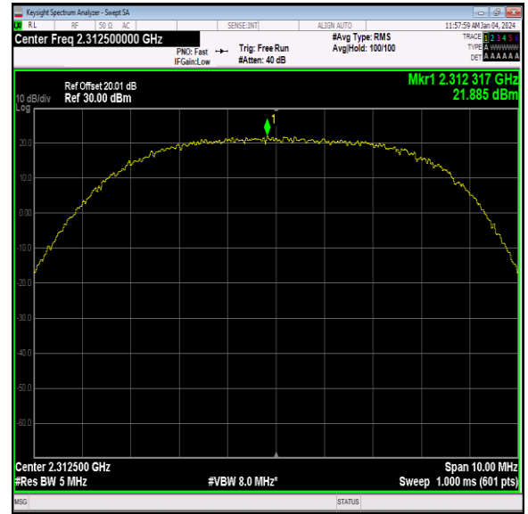
40(2305-2315)-5MHz-64QAM-38775-1RB#12-PASS
