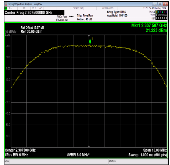
40(2305-2315)-5MHz-64QAM-38725-1RB#12-PASS
