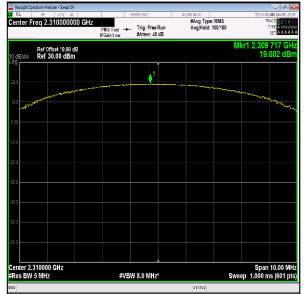
40(2305-2315)-5MHz-64QAM-38750-25RB#0-PASS
