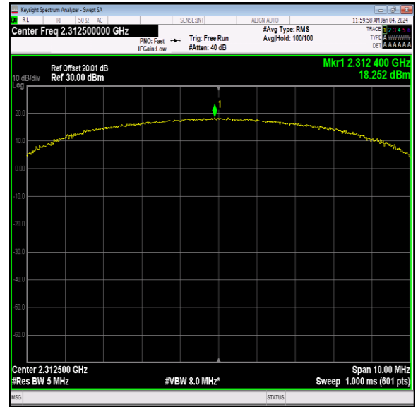
40(2305-2315)-5MHz-16QAM-38775-25RB#0-PASS
