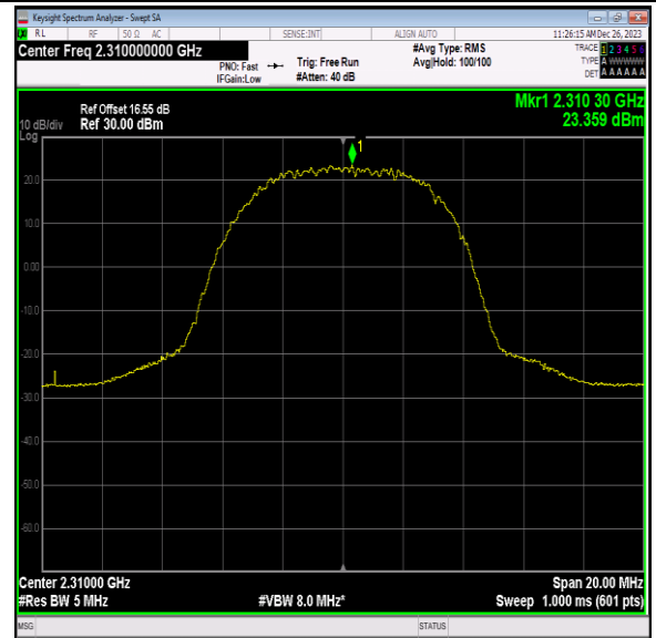
40(2305-2315)-10MHz-16QAM-38750-1RB#24-PASS
