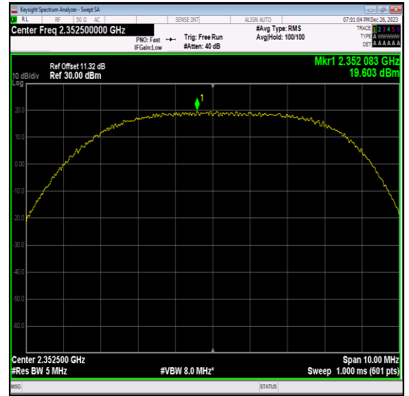
40(2350-2360)-5MHz-QPSK-39175-1RB#12-PASS
