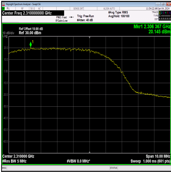
40(2305-2315)-5MHz-16QAM-38750-1RB#0-PASS
