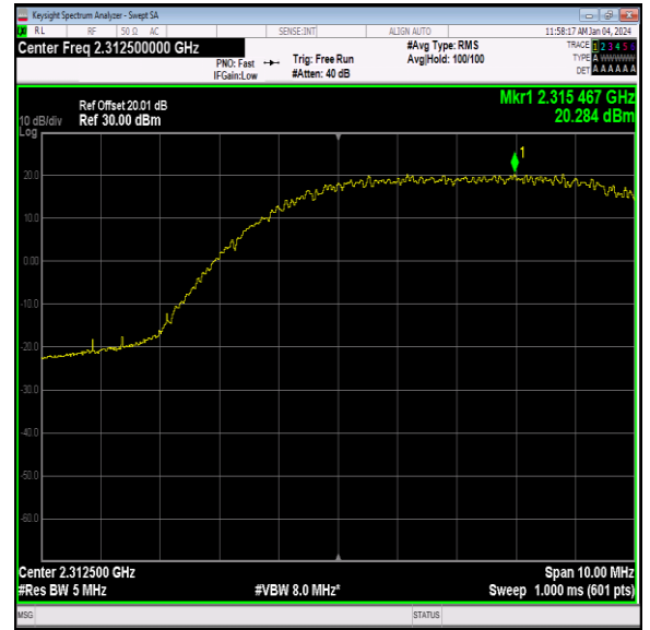
40(2305-2315)-5MHz-16QAM-38775-1RB#24-PASS
