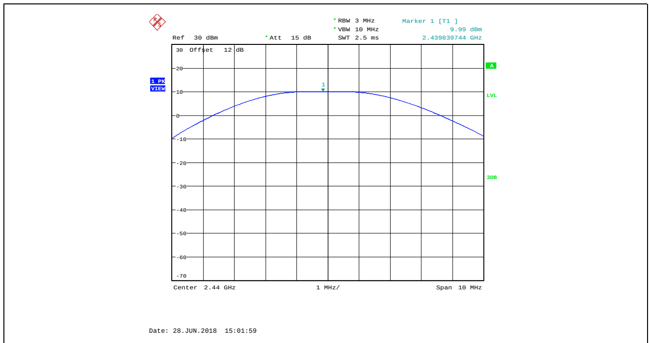
Plot 5.3.4.6. Maximum Peak Conducted Output Power, O-QPSK Modulation, Power Setting 107, Ch 18, 2440 MHz
