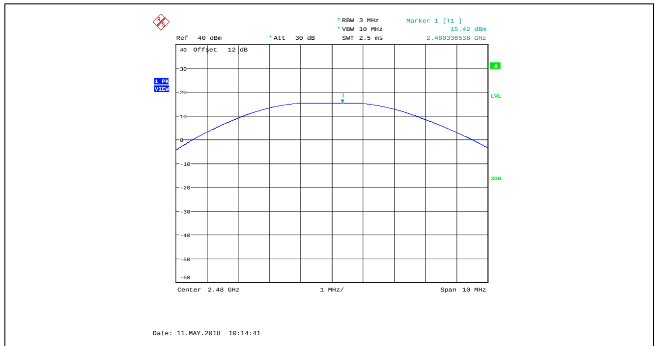
Plot 5.3.4.4. Maximum Peak Conducted Output Power, O-QPSK Modulation, Power Setting 160, Ch 26, 2480 MHz
