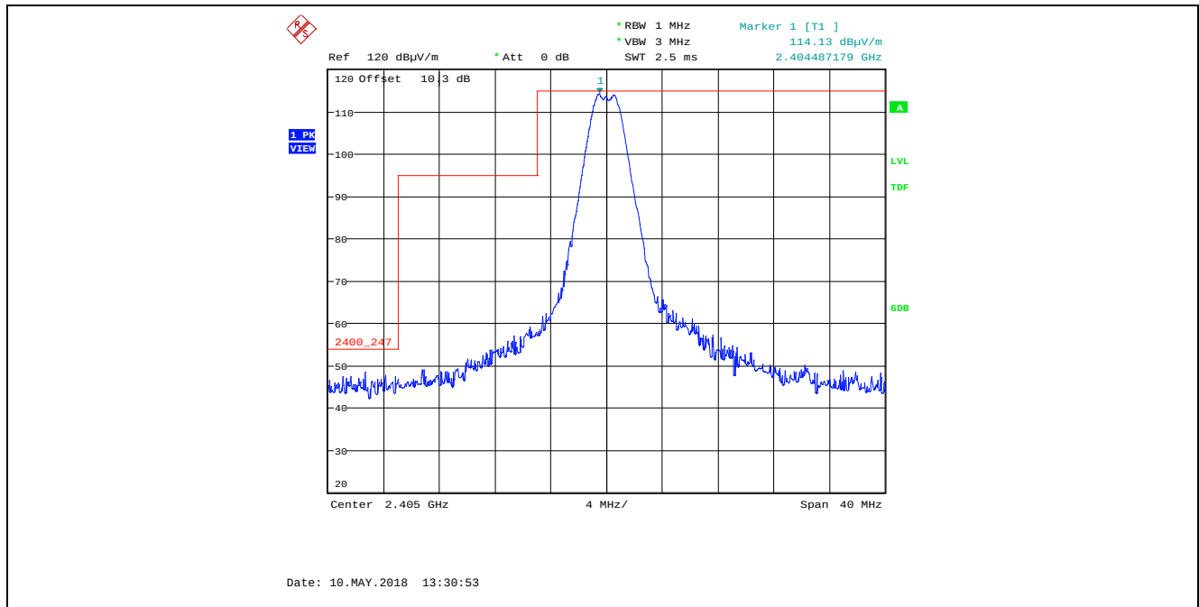
Plot 5.4.4.3.1. Band-Edge Radiated Emissions, EUT with 1.72 dBi Chip Antenna, Lower Band-edge Rx Antenna in Vertical Polarization, O-QPSK Modulation, Power Setting 200, Ch 11, 2405 MHz
