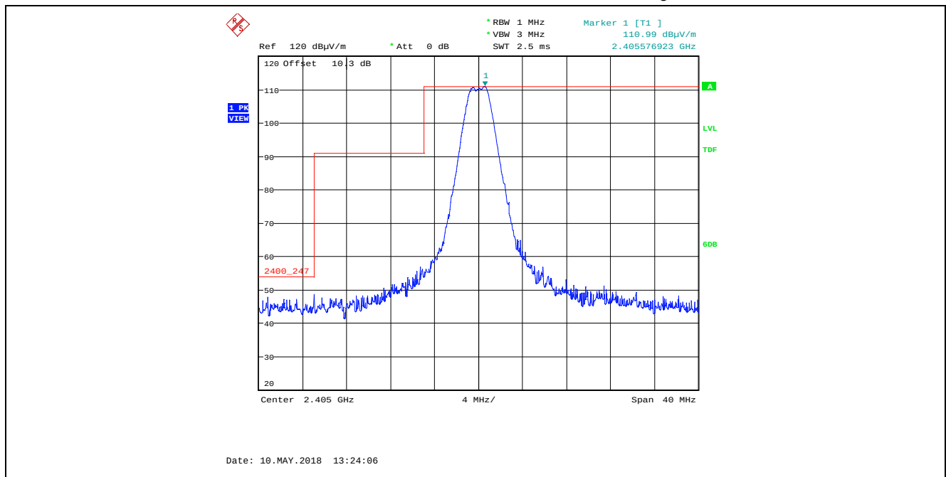
Plot 5.4.4.3.2. Band-Edge Radiated Emissions, EUT with 1.72 dBi Chip Antenna, Lower Band-edge Rx Antenna in Horizontal Polarization, O-QPSK Modulation, Power Setting 200, Ch 11, 2405 MHz
