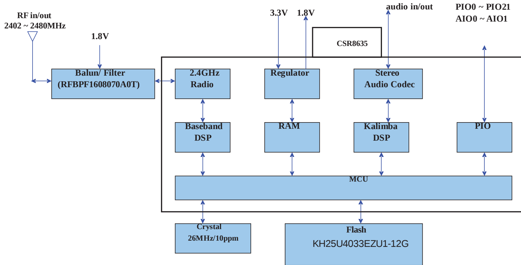
JS-BTM8635 Block Diagram
