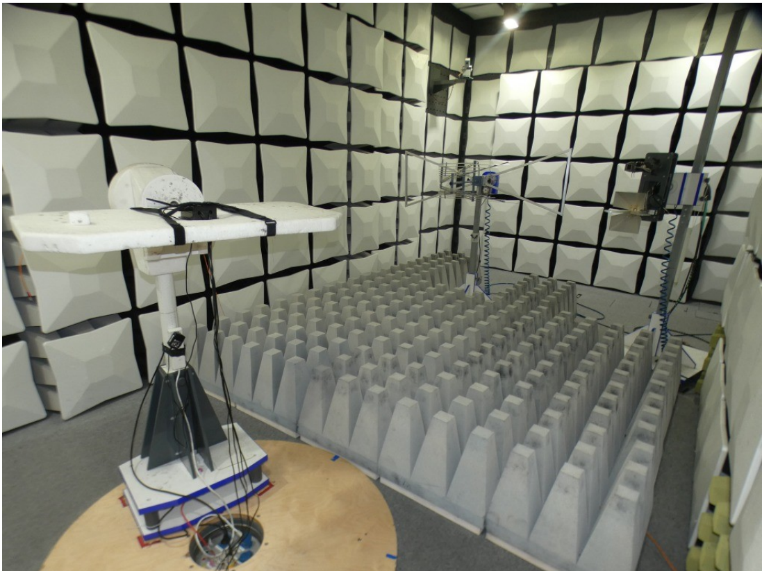
Photo 2: Test setup for radiated measurements above 1 GHz
