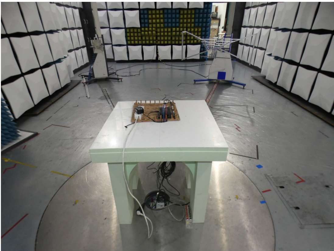
Test setup for radiated measurements below 1 GHz
