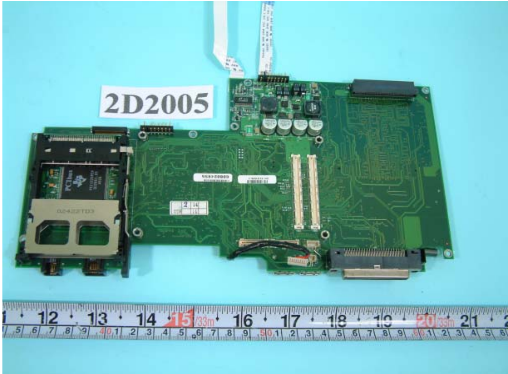
Rear side of main board
