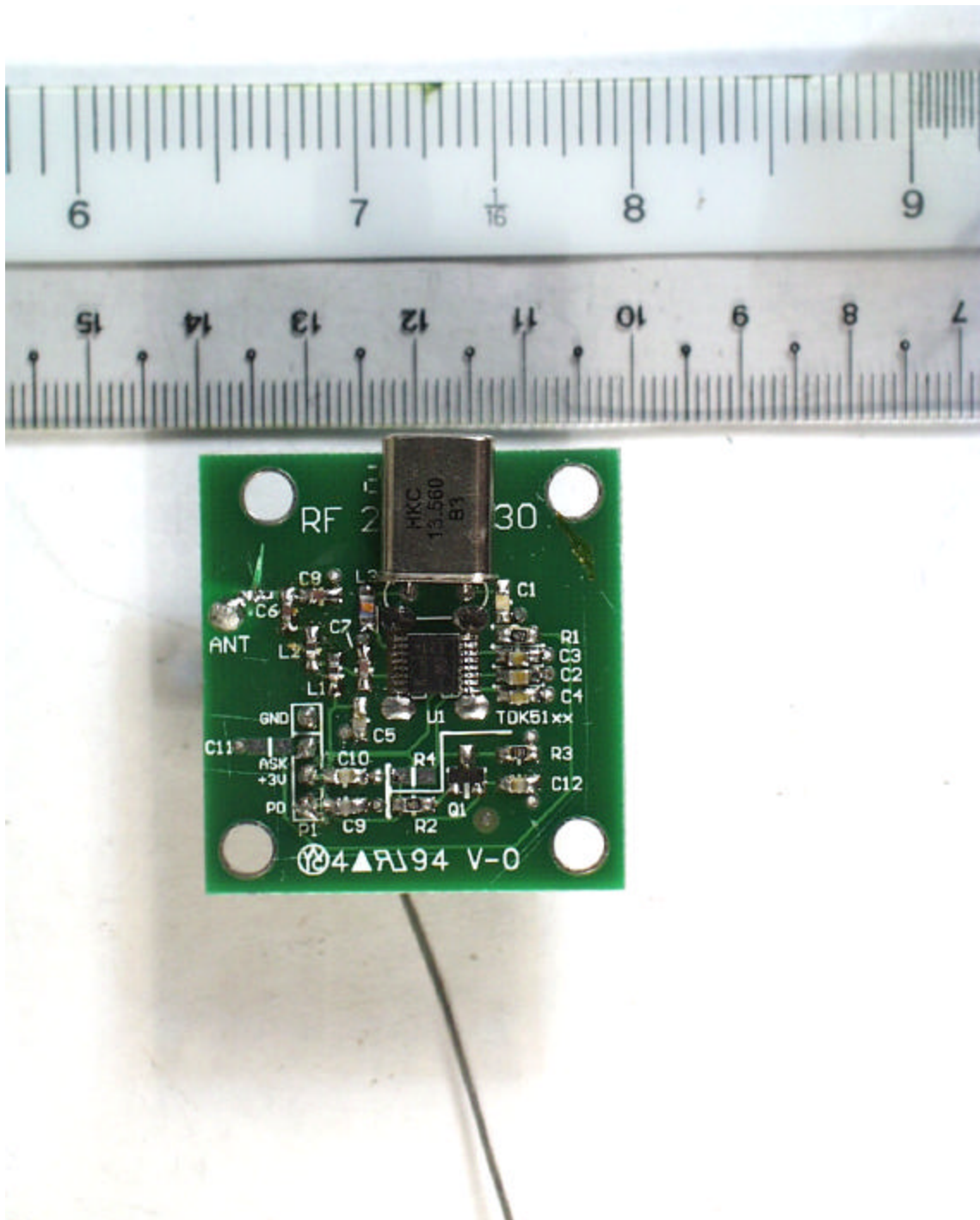
Component Side (RF Module) – RF Remote Controller
