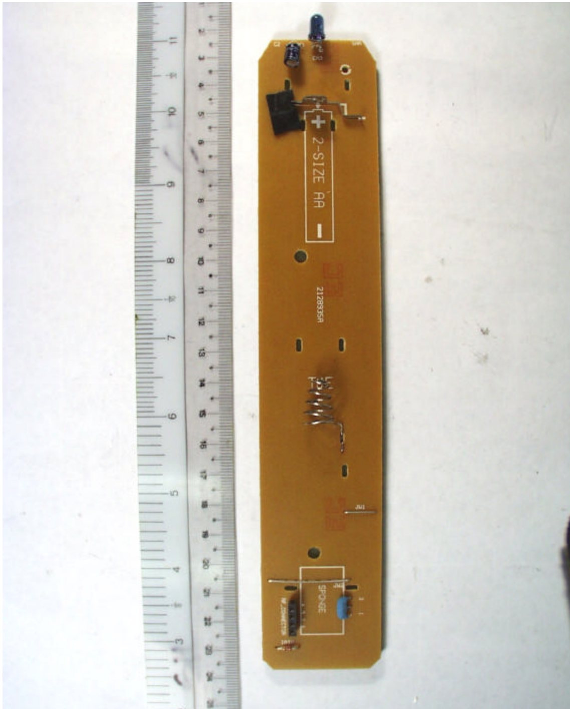
Component Side (Main PCB) – RF Remote Controller
