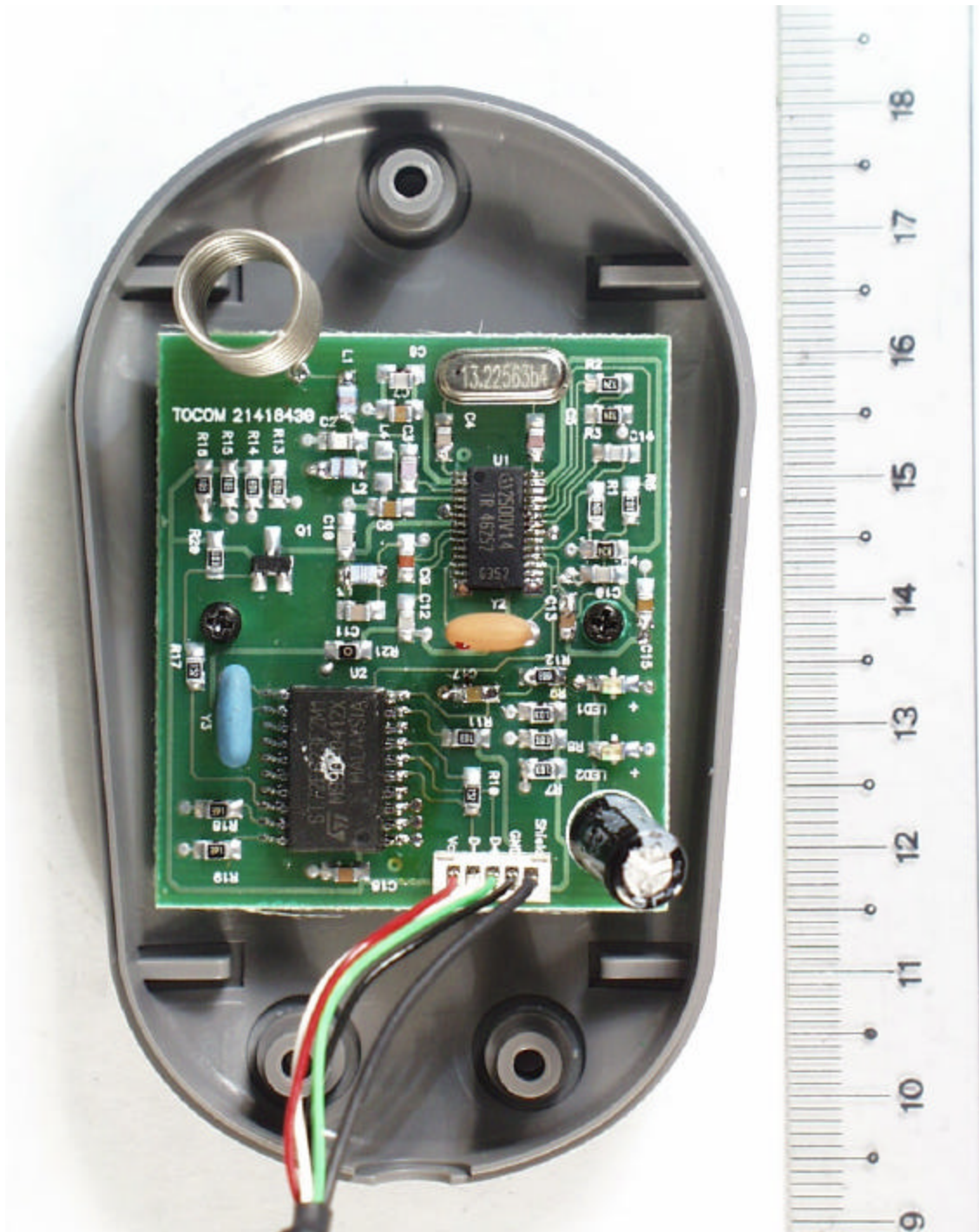
Overall Internal View – RF Dongle
