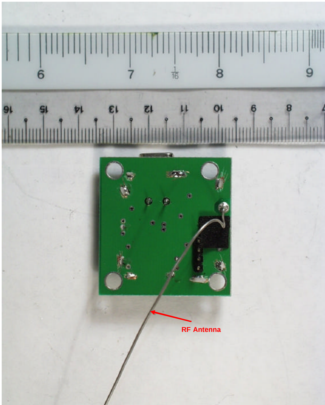
Trace Side (RF Module) – RF Remote Controller
