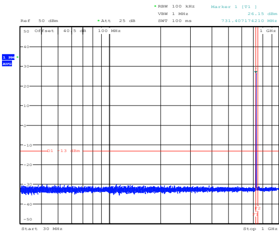
Figure 8.4-1: Conducted spurious emissions below 1 GHz for low channel (SMR700)
