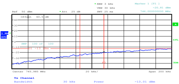
Figure 8.4-24: Conducted lower band edge at 746 MHz at AGC threshold + 3 dB (LTE700)
