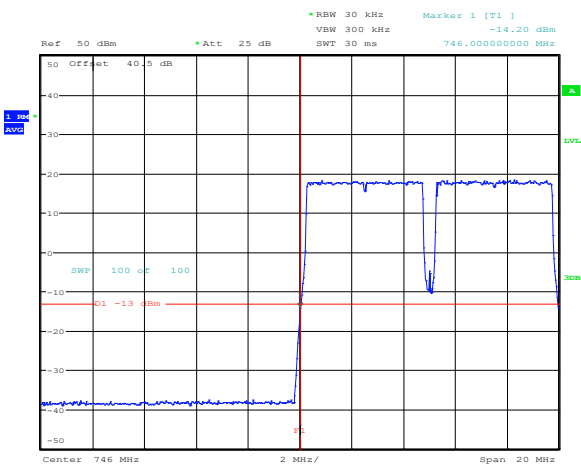
Figure 8.4-39: Conducted lower band edge at 746 MHz at AGC threshold (intermodulation) (LTE700)
