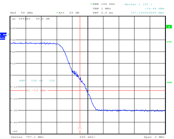
Figure 8.4-32: Conducted upper band edge at 758 MHz at AGC threshold + 3 dB (LTE700)
