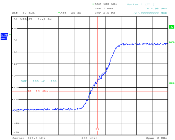
Figure 8.4-20: Conducted lower band edge at 728 MHz at AGC threshold + 3 dB (SMR700)
