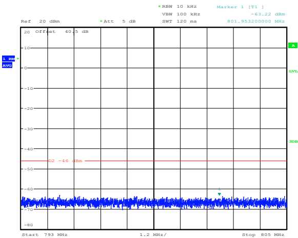
Figure 8.4-13: Conducted spurious emissions 793-805 MHz for low channel (LTE700)
