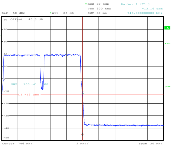
Figure 8.4-44: Conducted upper band edge at 746 MHz at AGC threshold + 3 dB (intermodulation) (SMR700)
