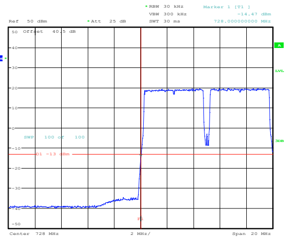
Figure 8.4-36: Conducted lower band edge at 728 MHz at AGC threshold + 3 dB (intermodulation) (SMR700)
