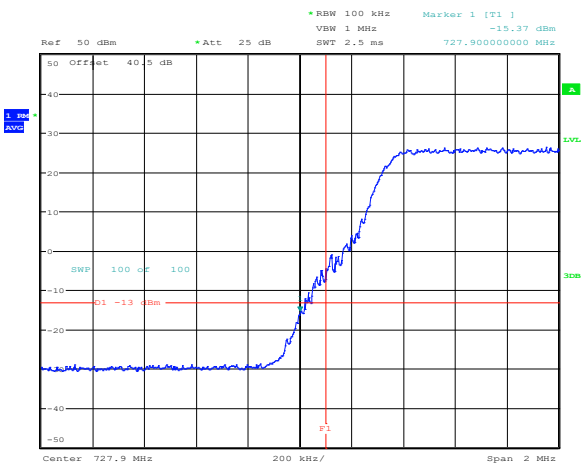
Figure 8.4-19: Conducted lower band edge at 728 MHz at AGC threshold (SMR700)
