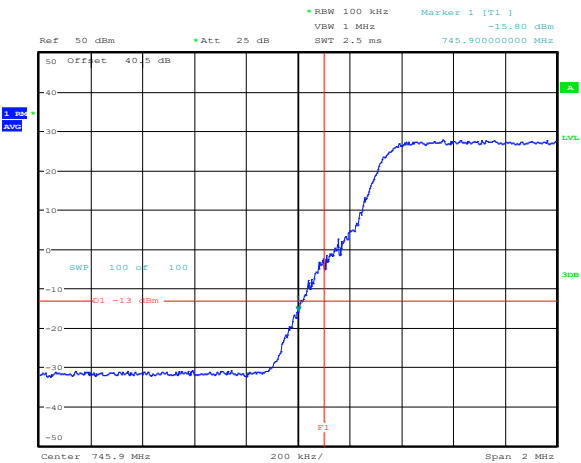
Figure 8.4-24: Conducted lower band edge at 746 MHz at AGC threshold + 3 dB (LTE700)
