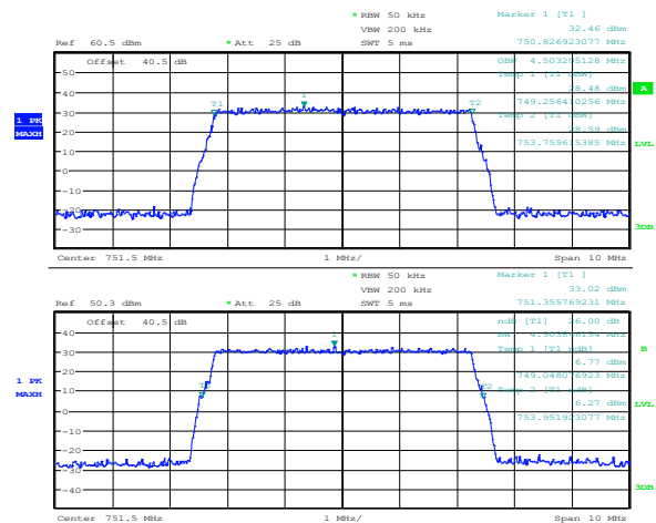
Figure 8.6-18: 99% OBW and 26 dB EBW at the output of the EUT at AGC threshold, Middle channel (LTE700)
