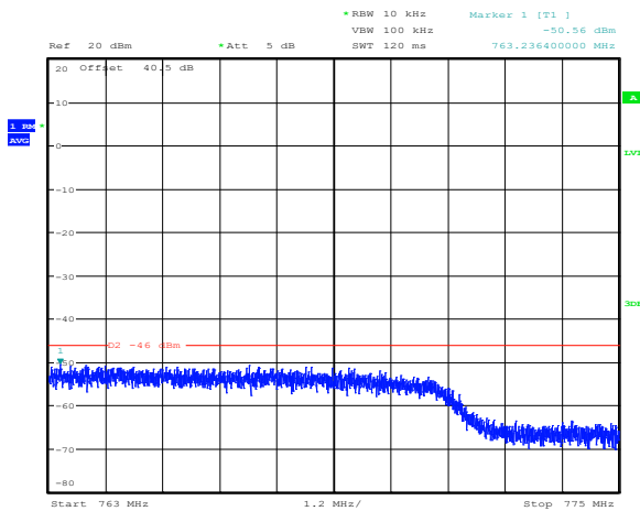
Figure 8.4-17: Conducted spurious emissions 763-775 MHz for mid channel (LTE700)
