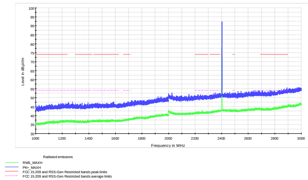
Figure 8.6-31: Radiated spurious emissions within 1–3 GHz at low channel
