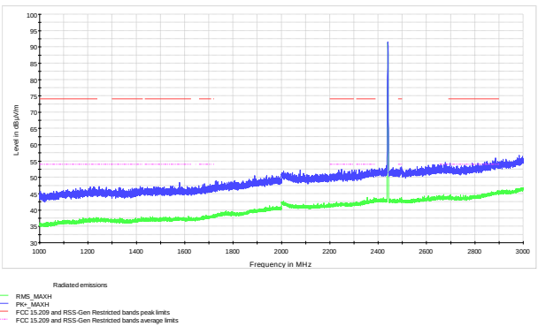
Figure 8.6-32: Radiated spurious emissions within 1–3 GHz at mid channel
