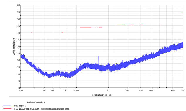
Figure 8.6-27: Radiated spurious emissions below 1 GHz at low channel
