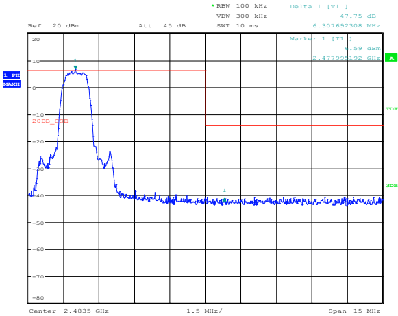
Figure 8.6-11: Conducted spurious emissions at the low upper edge for \pi/4 -DQPSK modulation, hopping off
