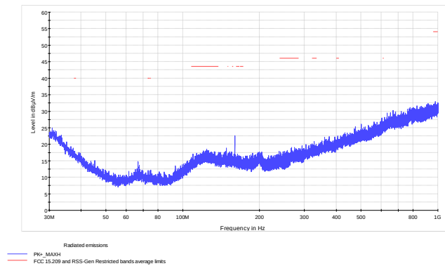
Figure 8.6-29: Radiated spurious emissions below 1 GHz at high channel
