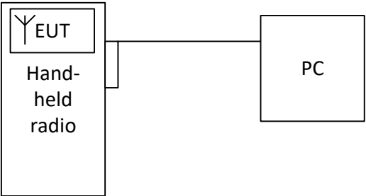
Figure 3.6-1: Setup diagram
