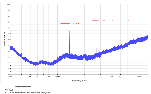
Figure 8.6-30: d spurious emissions below 1 GHz with VHF radio turned on
