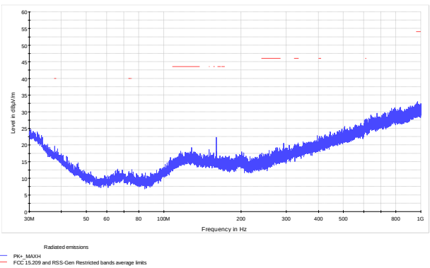
Figure 8.6-28: Radiated spurious emissions below 1 GHz at mid channel
