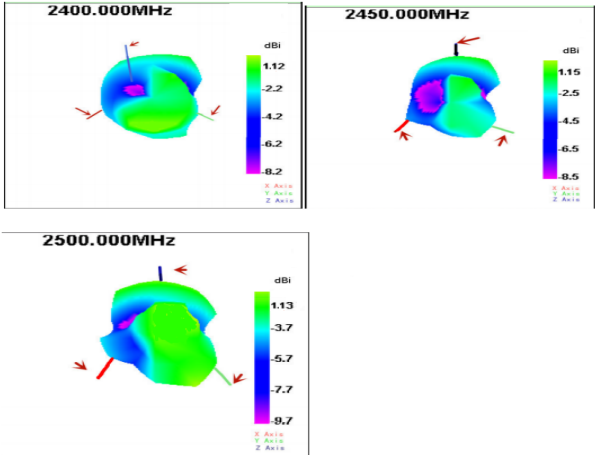
方向图/ Directional map:
