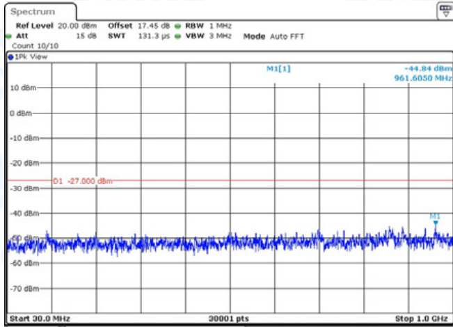
11N20-CDD-Ant1-5180-30~1000-PASS
