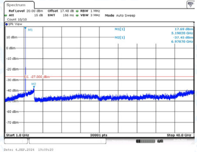
11A-Ant2-5200-1000~40000-PASS
