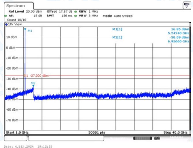
11A-Ant2-5240-1000~40000-PASS
