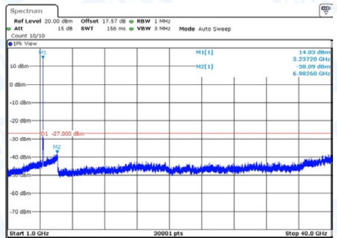
11N20-CDD-Ant1-5240-1000~40000-PASS
