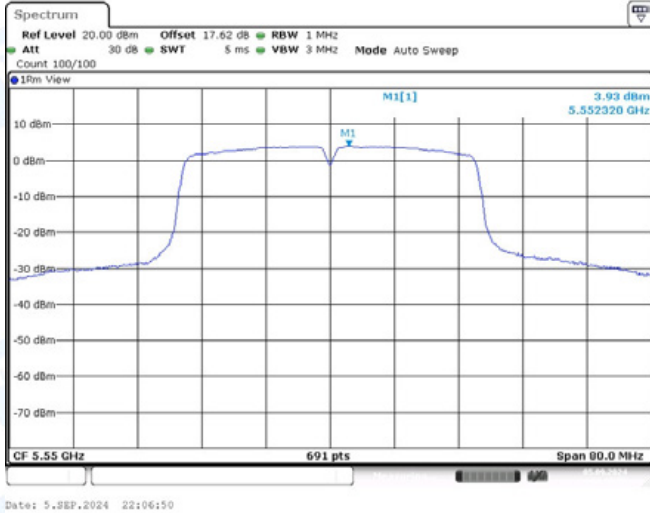
11AC40-CDD-Ant1-5550-PASS
