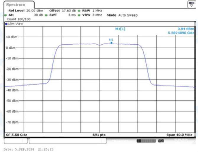
11AC20-CDD-Ant2-5580-PASS
