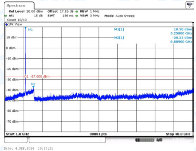
11A-Ant2-5260-1000~40000-PASS
