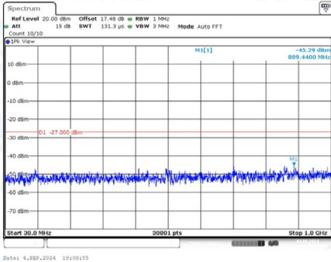
11A-Ant2-5200-30~1000-PASS
