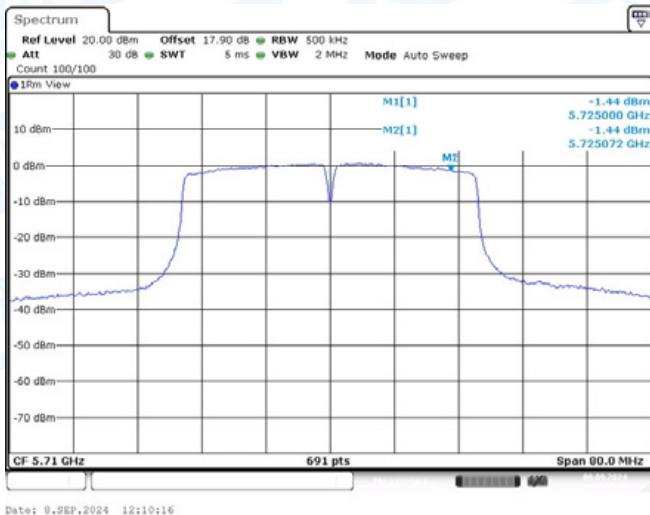
11AC40-CDD-Ant1-5710_UNII-3-PASS
