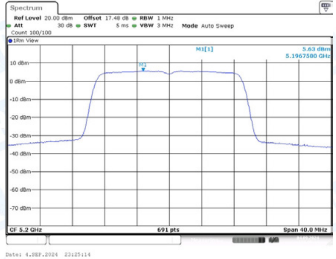
11AC20-CDD-Ant2-5200-PASS
