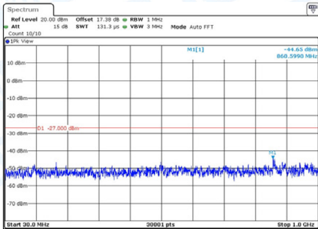
11N20-CDD-Ant2-5180-30~1000-PASS
