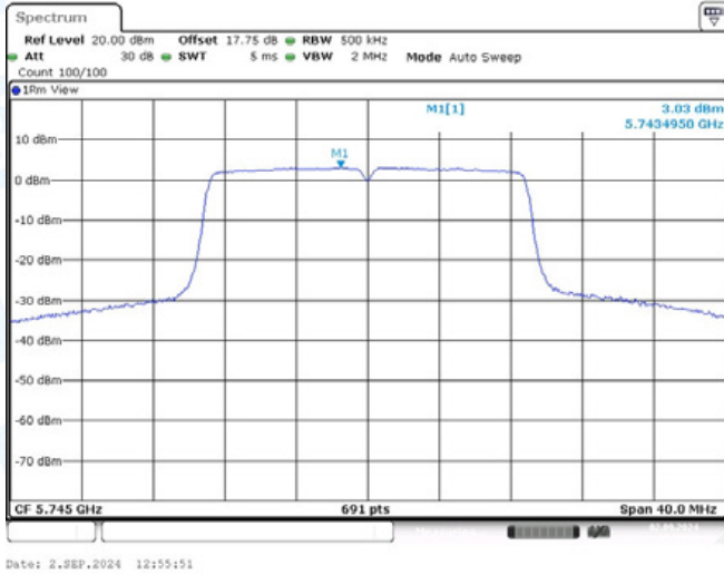
11AC20-CDD-Ant1-5745-PASS
