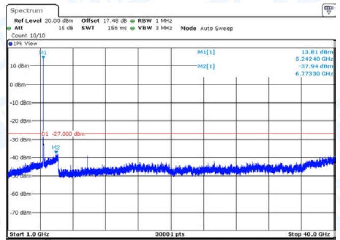
11N20-CDD-Ant2-5200-1000~40000-PASS
