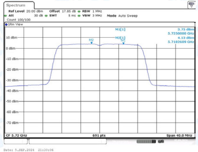
11AC20-CDD-Ant2-5720_UNII-2C-PASS
