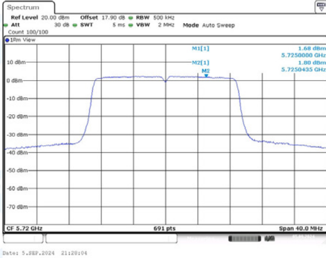
11AC20-CDD-Ant1-5720_UNII-3-PASS
