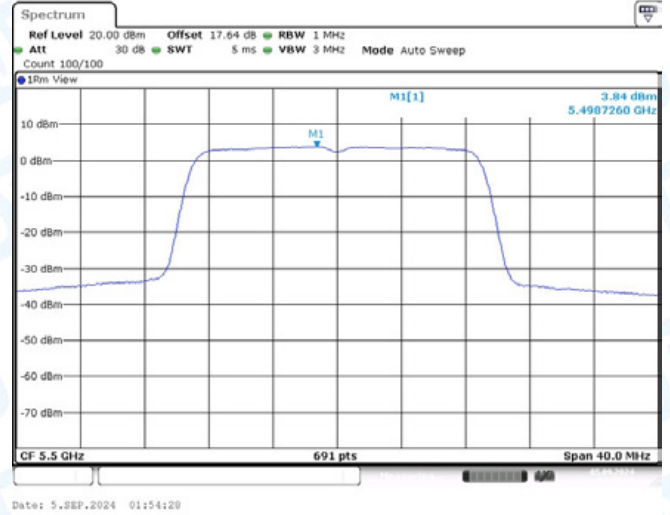
11AC20-CDD-Ant2-5500-PASS
