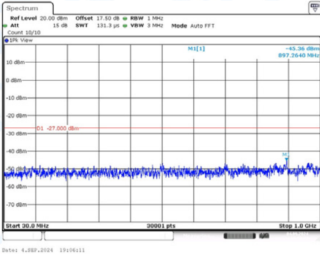
11A-Ant2-5180-30~1000-PASS
