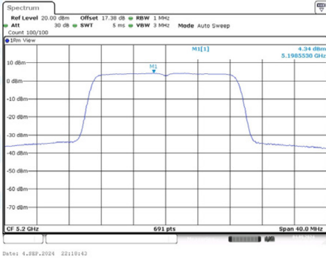
11AC20-CDD-Ant1-5200-PASS
