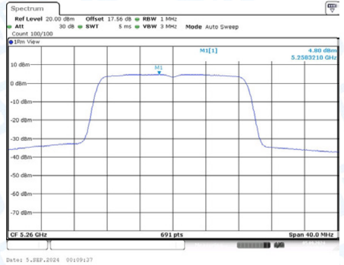
11AC20-CDD-Ant2-5260-PASS
