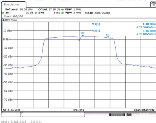
11AC40-CDD-Ant1-5710_UNII-2C-PASS
