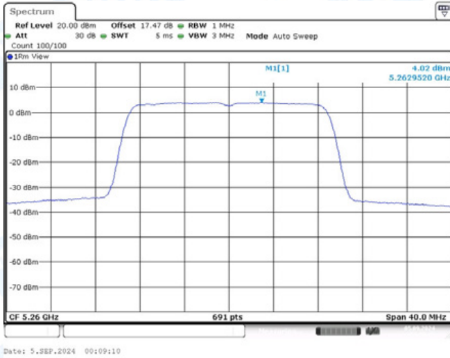
11AC20-CDD-Ant1-5260-PASS
