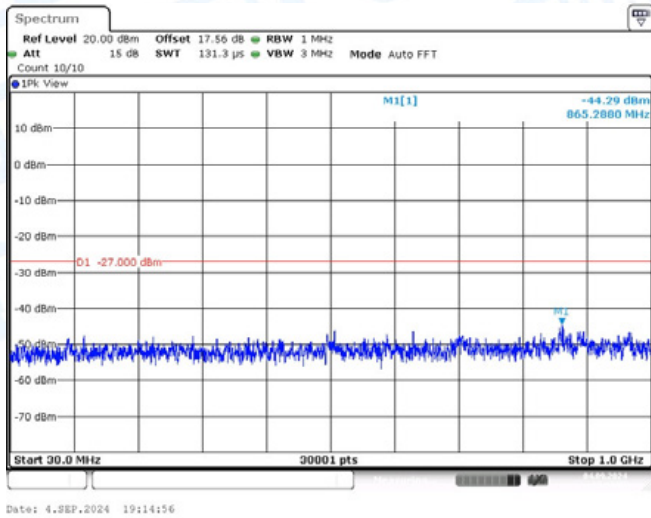
11A-Ant2-5260-30~1000-PASS
