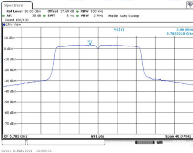
11AC20-CDD-Ant1-5785-PASS
