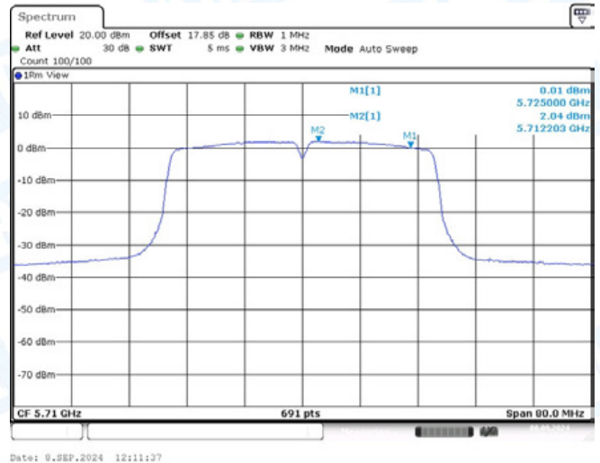
11AC40-CDD-Ant2-5710_UNII-2C-PASS
