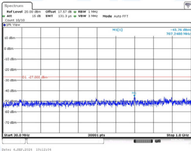
11A-Ant2-5240-30~1000-PASS
