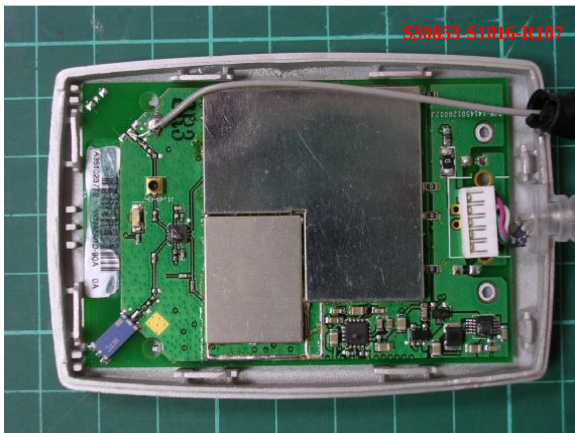
Photo 1: Internal photo of EUT (Type 1 antenna)
