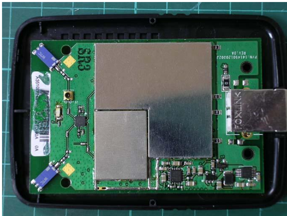
Photo 5: Internal photo of ST120g (Type 2 antenna)
