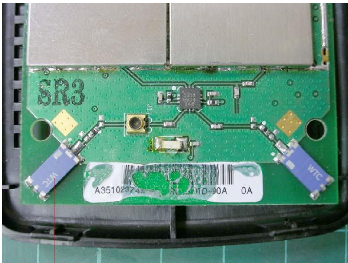
Photo 6: Internal photo of ST120g (Type 2 antenna)
