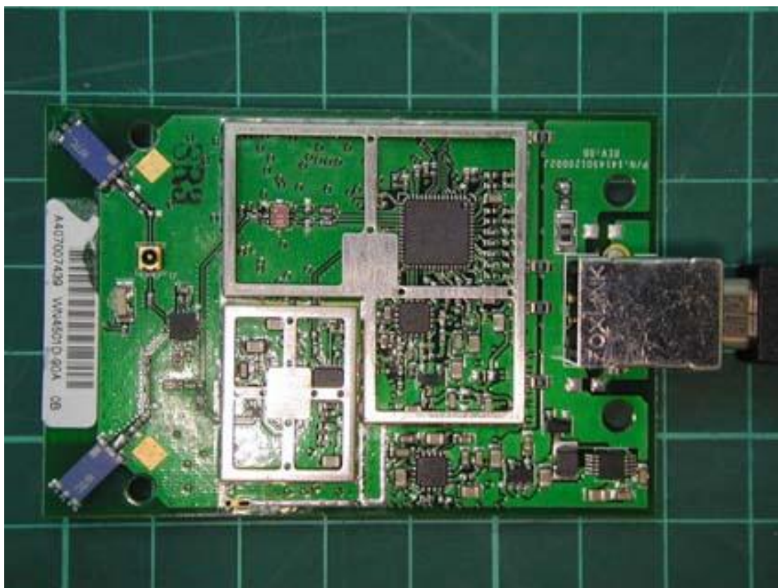
Photo 7: Internal photo of ST120g (Type 2 antenna)
