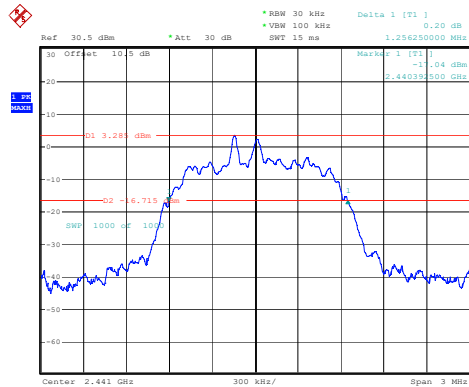
2DH1_Middle 1.256MHz
