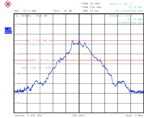
DH1_Middle 0.941MHz
