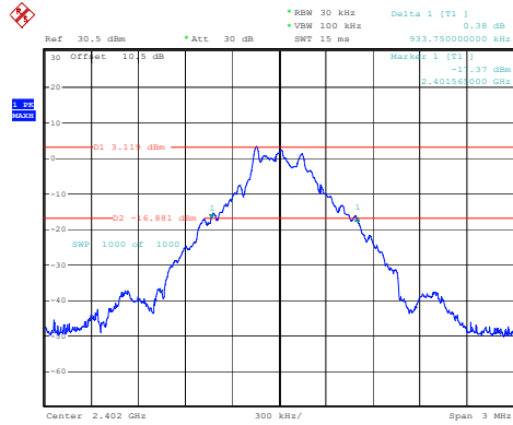
DH1_Low 0.934MHz
