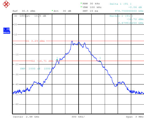
DH1_High 0.979MHz
