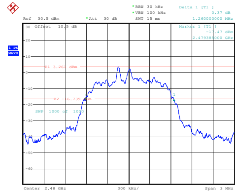
2DH1_High 1.260MHz
