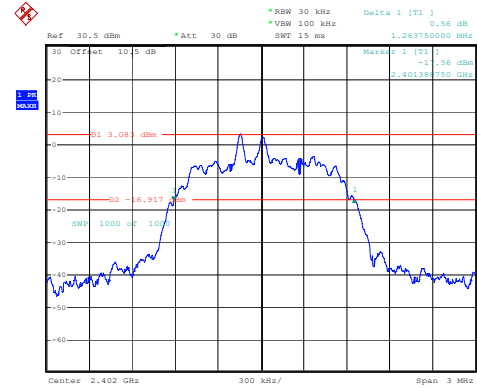
2DH1_Low 1.264MHz
