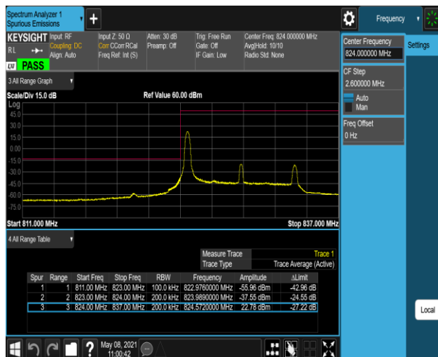
Band5-10MHz-QPSK-20450-50RB#0
