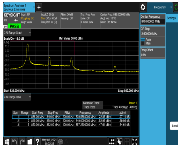
Band5-10MHz-QPSK-20600-50RB#0
