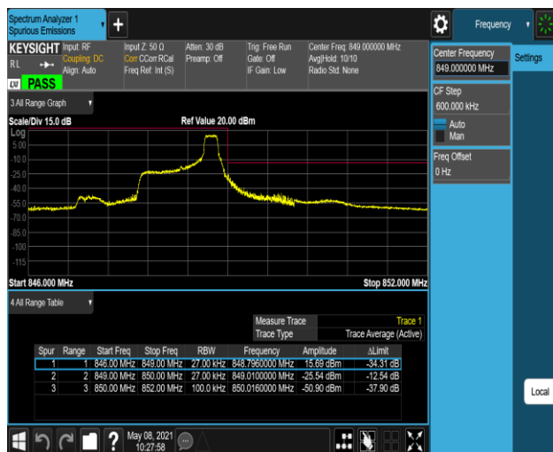
Band5-1.4MHz-16QAM-20643-1RB#5
