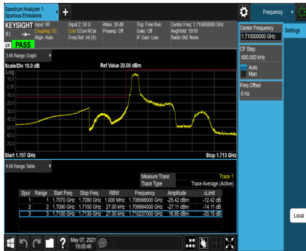
Band4-1.4MHz-QPSK-19957-6RB#0
