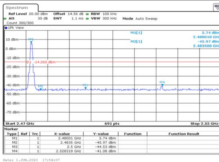
LE 1M_Ant1_High_2480
