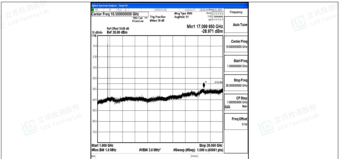
Band7_5MHz_16QAM_21425_1RB#0_1000~20000_1000~20000
