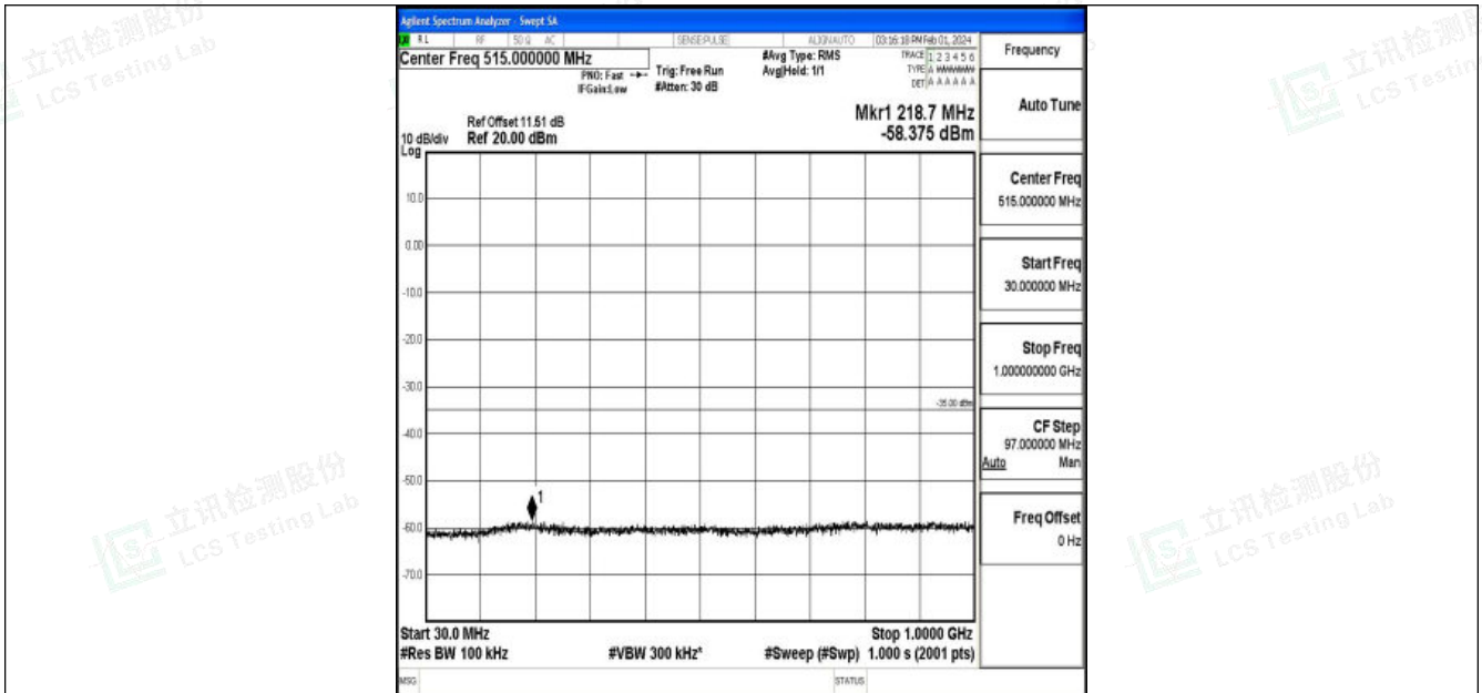
Band7_20MHz_QPSK_21100_1RB#0_30~1000_30~1000
