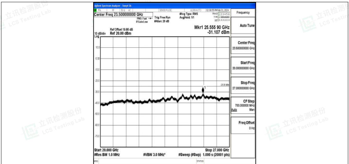
Band7_10MHz_QPSK_21100_1RB#0_20000~27000_20000~27000
