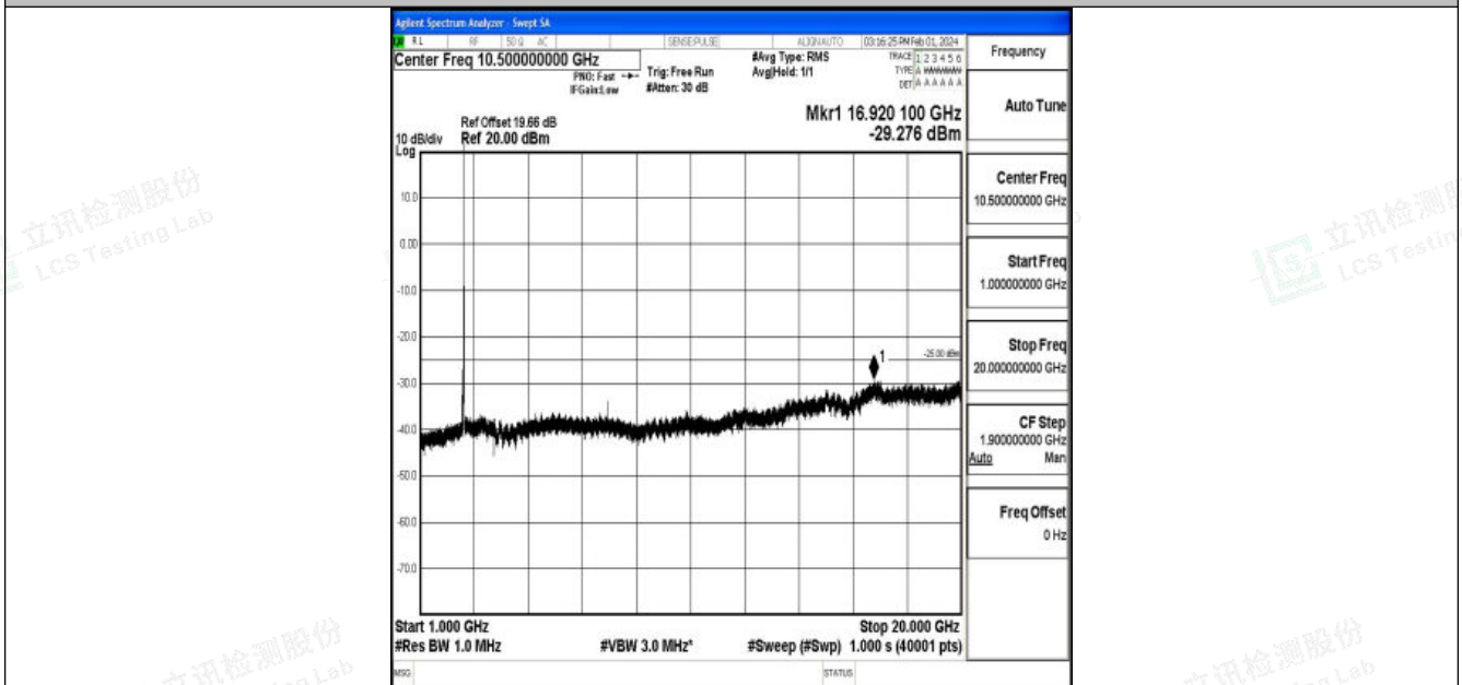
Band7_20MHz_QPSK_21100_1RB#0_1000~20000_1000~20000
