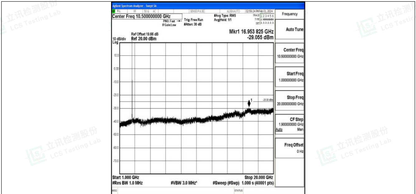
Band7_15MHz_16QAM_21375_1RB#0_1000~20000_1000~20000
