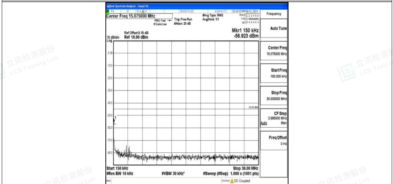
Band7_5MHz_QPSK_21100_1RB#0_0.15~30_0.15~30
