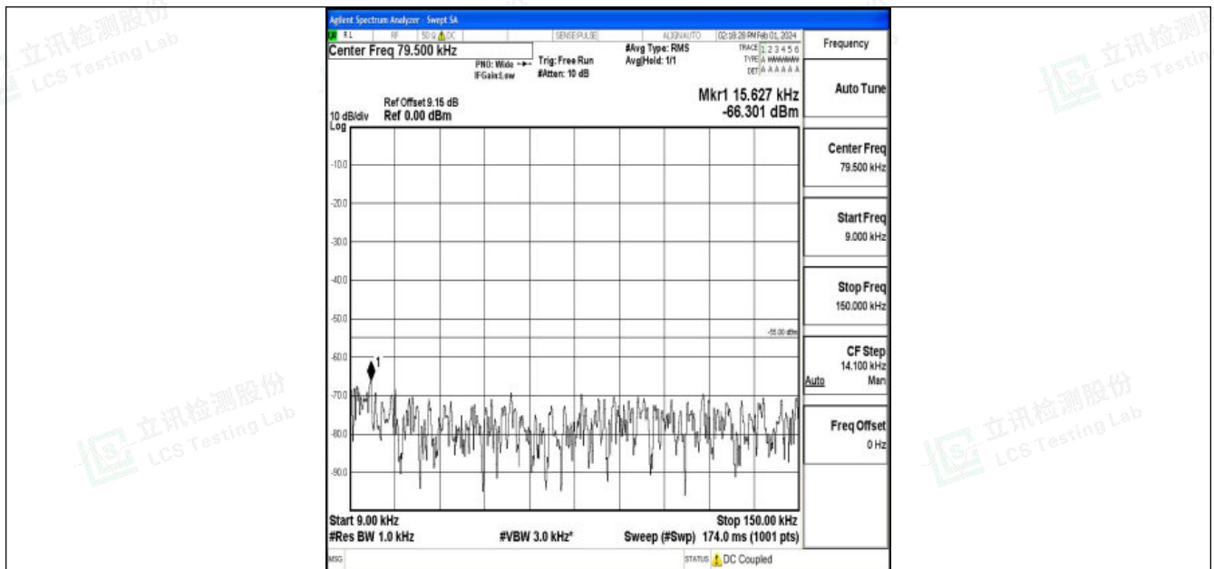
Band7_5MHz_QPSK_21100_1RB#0_0.009~0.15_0.009~0.15
