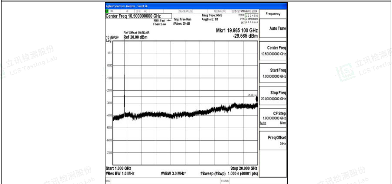
Band7_20MHz_QPSK_21350_1RB#0_1000~20000_1000~20000
