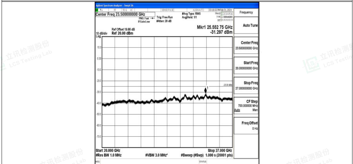
Band7_20MHz_16QAM_21350_1RB#0_20000~27000_20000~27000
