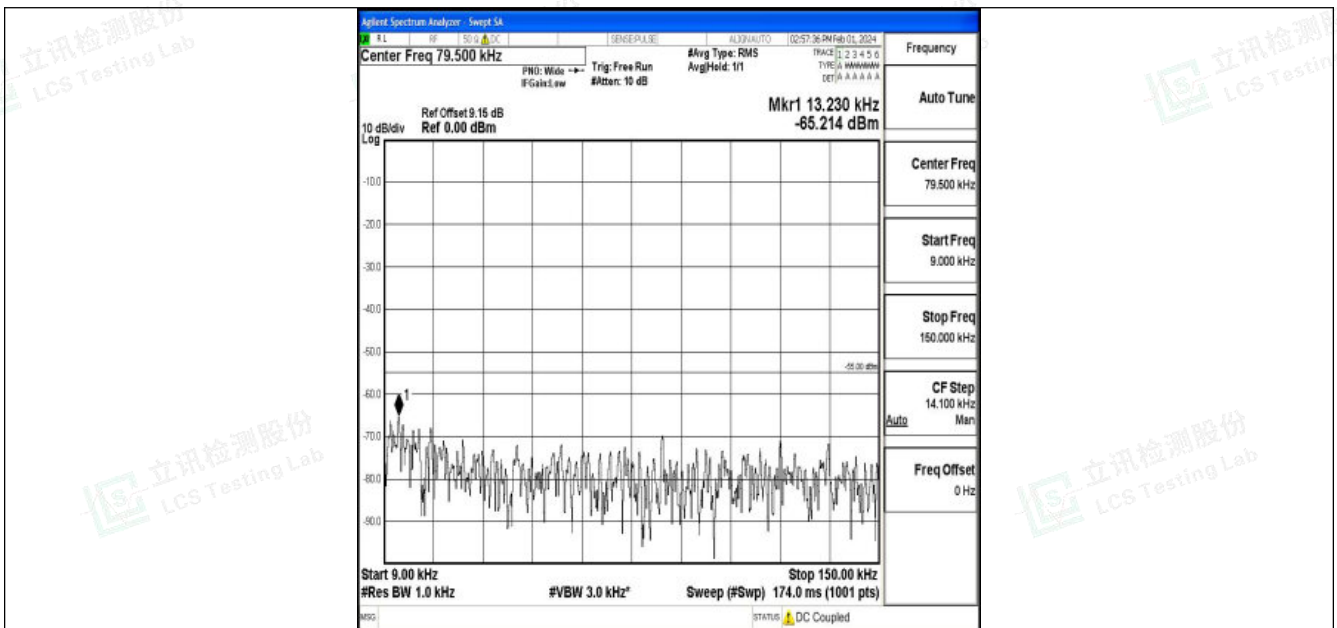
Band7_15MHz_QPSK_21100_1RB#0_0.009~0.15_0.009~0.15
