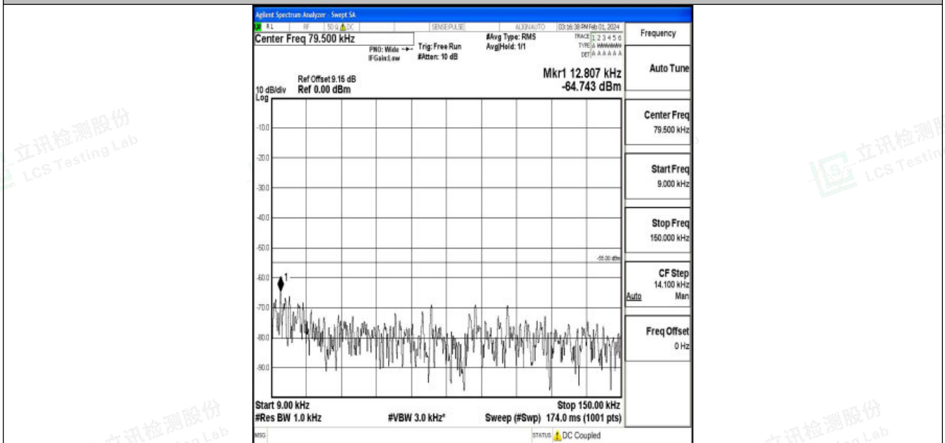
Band7_20MHz_16QAM_21100_1RB#0_0.009~0.15_0.009~0.15
