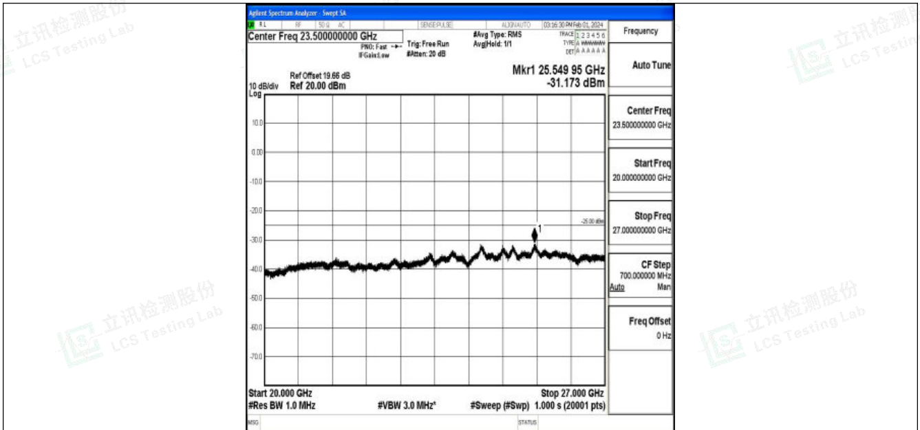
Band7_20MHz_QPSK_21100_1RB#0_20000~27000_20000~27000
