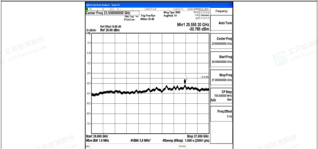
Band7_5MHz_16QAM_21425_1RB#0_20000~27000_20000~27000
