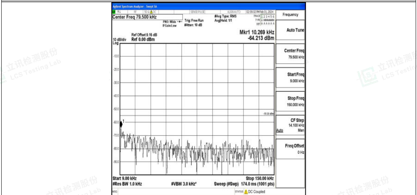
Band7_10MHz_16QAM_21100_1RB#0_0.009~0.15_0.009~0.15
