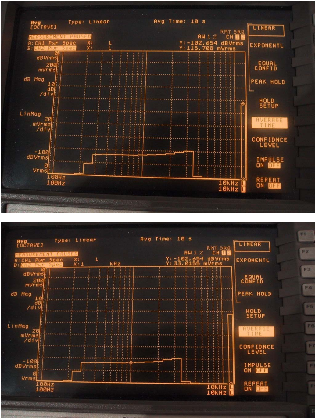
Figure 2: Top plot shows RMS time averaging power for the “48k_voice_300-3000” signal (sum of third-octave filters from 100 Hz to 10 kHz) and bottom plot is RMS power at 1 kHz third-octave filter.
